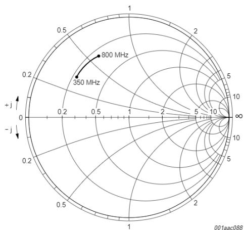
Fig 7. Input impedance ( s_{11} ) of the high band mixer (350 MHz to 800 MHz); Z_o = 100 \text{ }\Omega
