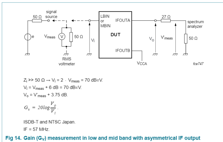
Fig 14. Gain ( G_v ) measurement in low and mid band with asymmetrical IF output
