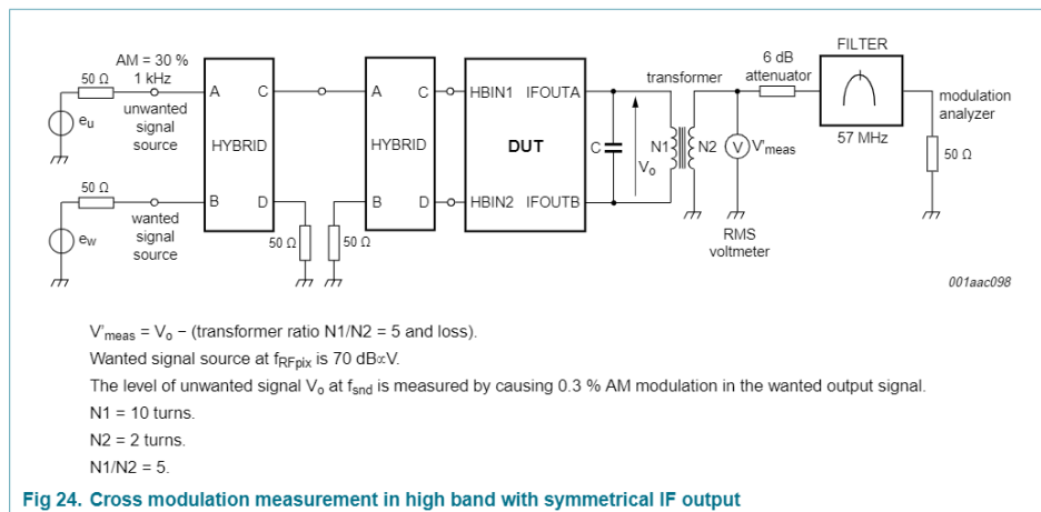
Fig 24. Cross modulation measurement in high band with symmetrical IF output
