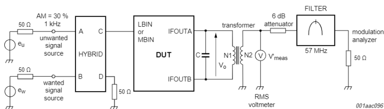
Fig 18. Cross modulation measurement in low and mid band with asymmetrical IF output
