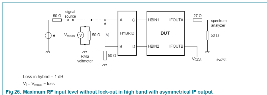
Fig 26. Maximum RF input level without lock-out in high band with asymmetrical IF output
