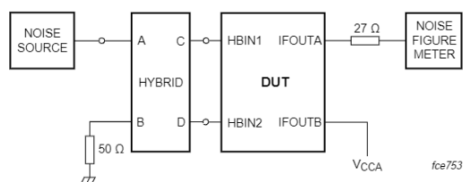
Fig 22. Noise figure (NF) measurement in high band with asymmetrical IF output
