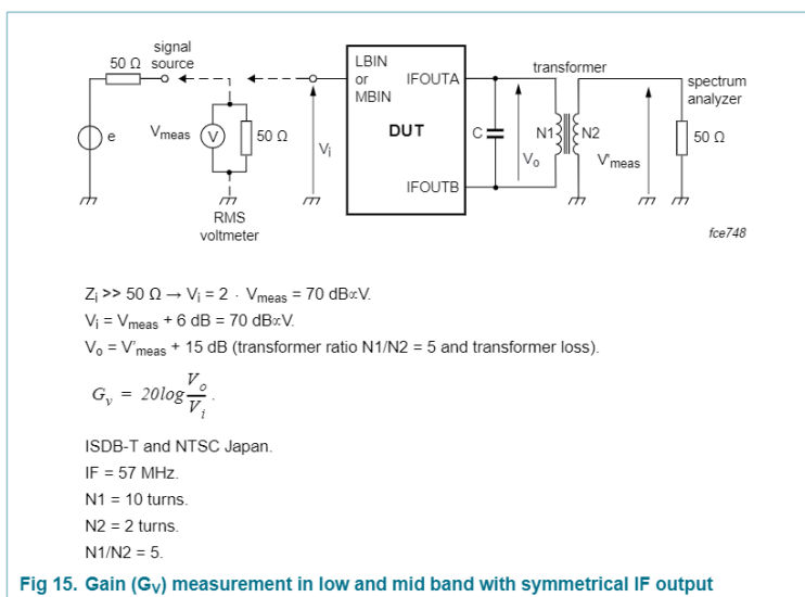
Fig 15. Gain ( G_v ) measurement in low and mid band with symmetrical IF output
