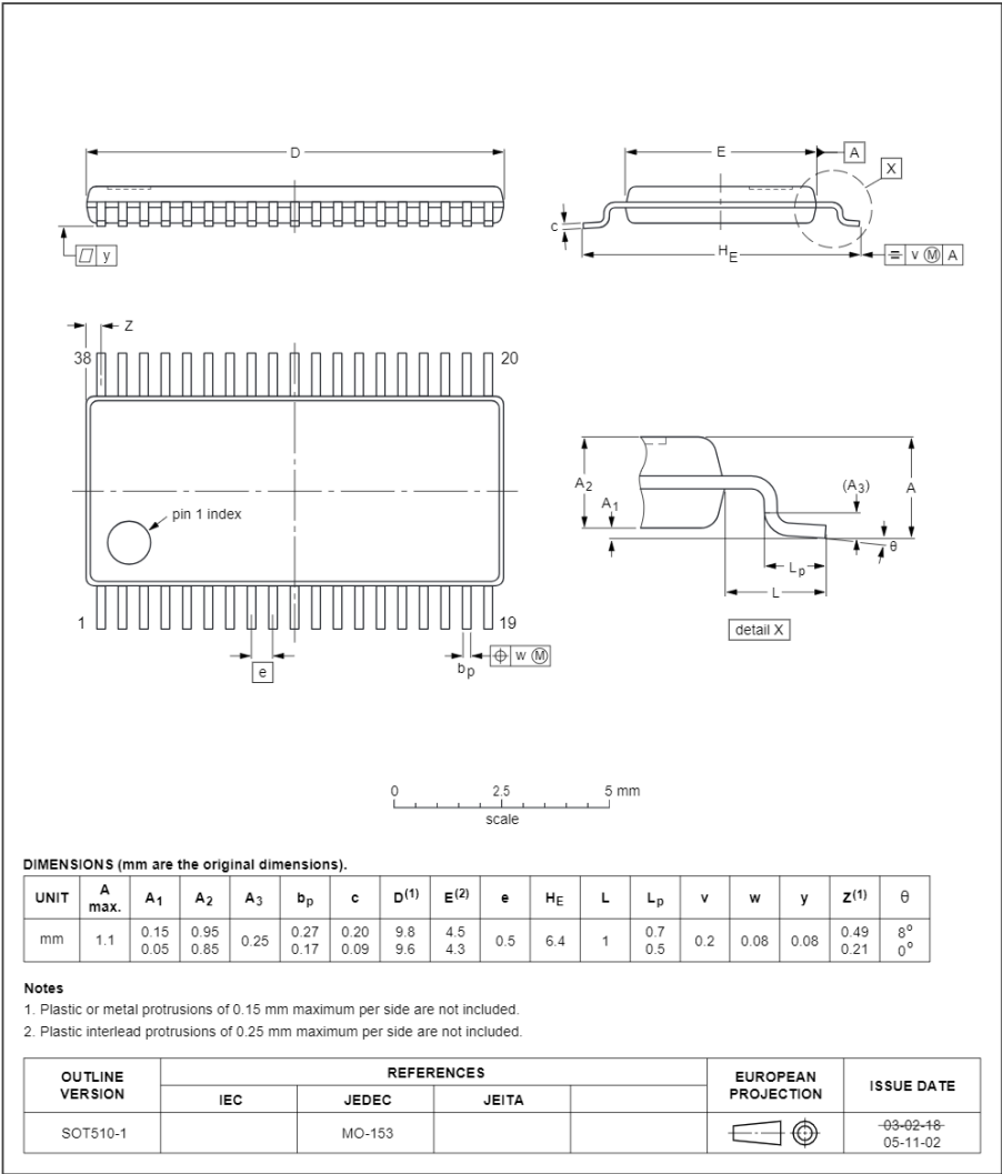
Fig 31. Package outline SOT510-1 (TSSOP38)
