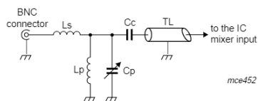
b. Schematic 2
