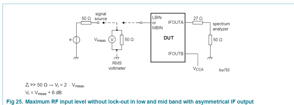
Fig 25. Maximum RF input level without lock-out in low and mid band with asymmetrical IF output
