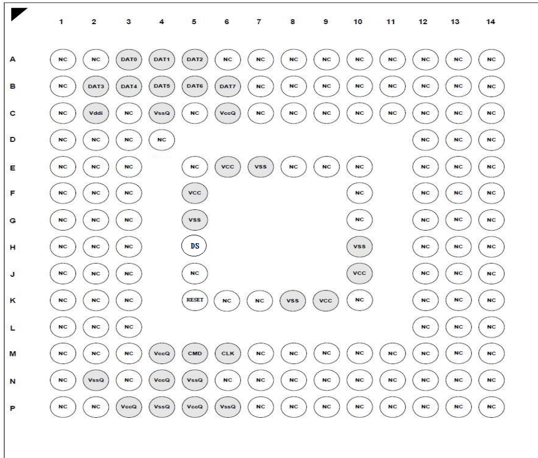
Figure 6 - FBGA153 Package Connection (top view through package)
