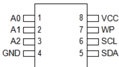
SOP-8/DIP-8/MSOP-8
