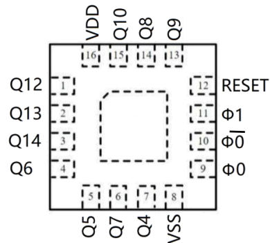
QFN-16 3*3
