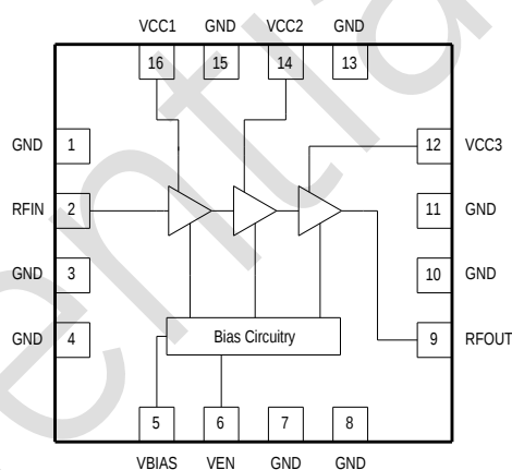
Figure 2. GDM2128 Function Block Diagram
