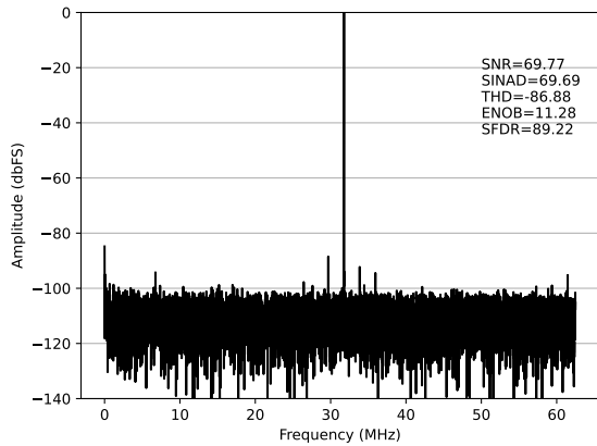
(c) 输入信号频率 = 31MHz
