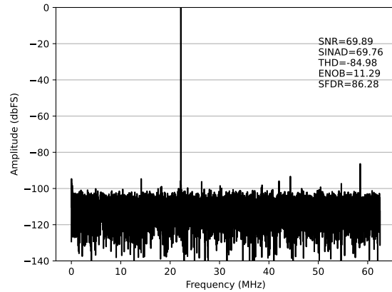
(b) 输入信号频率 = 22MHz
