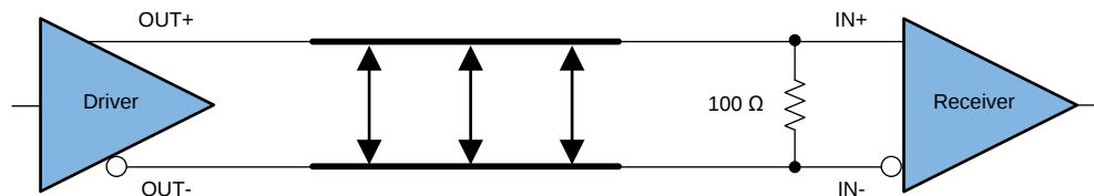
Figure 11. Point-to-Point Topology
