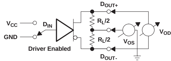
Figure 3. Driver V_{OD} and V_{OS} Test Circuit
