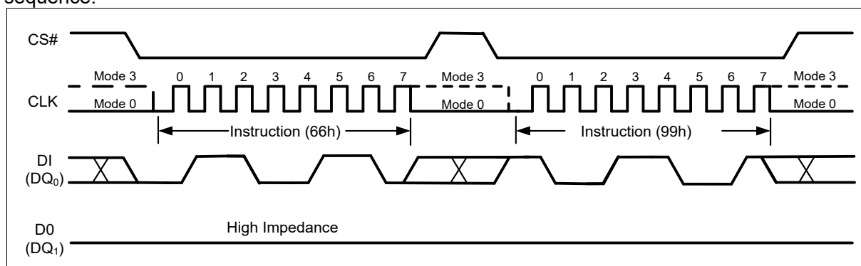
Figure 41 Enable Reset and Reset Instruction Sequence (SPI Mode)
