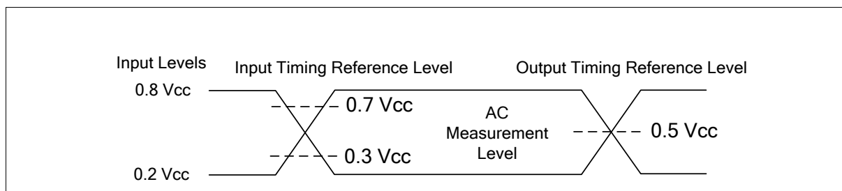
Figure 43 AC Measurement I/O Waveform
