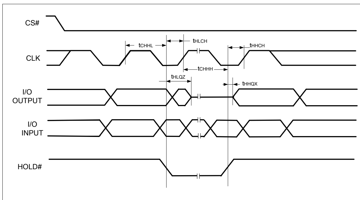
Figure 46 Hold Timing
