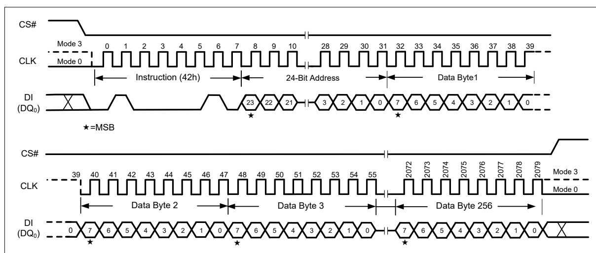
Figure 39 Program Security Sectors Instruction (SPI Mode)
