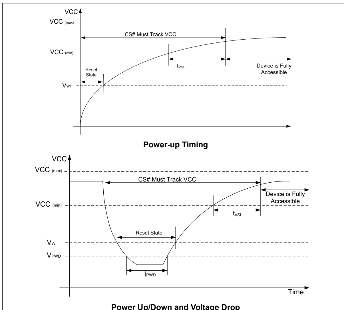
Figure 42 Power-up Timing &amp; Power Up/Down and Voltage Drop
