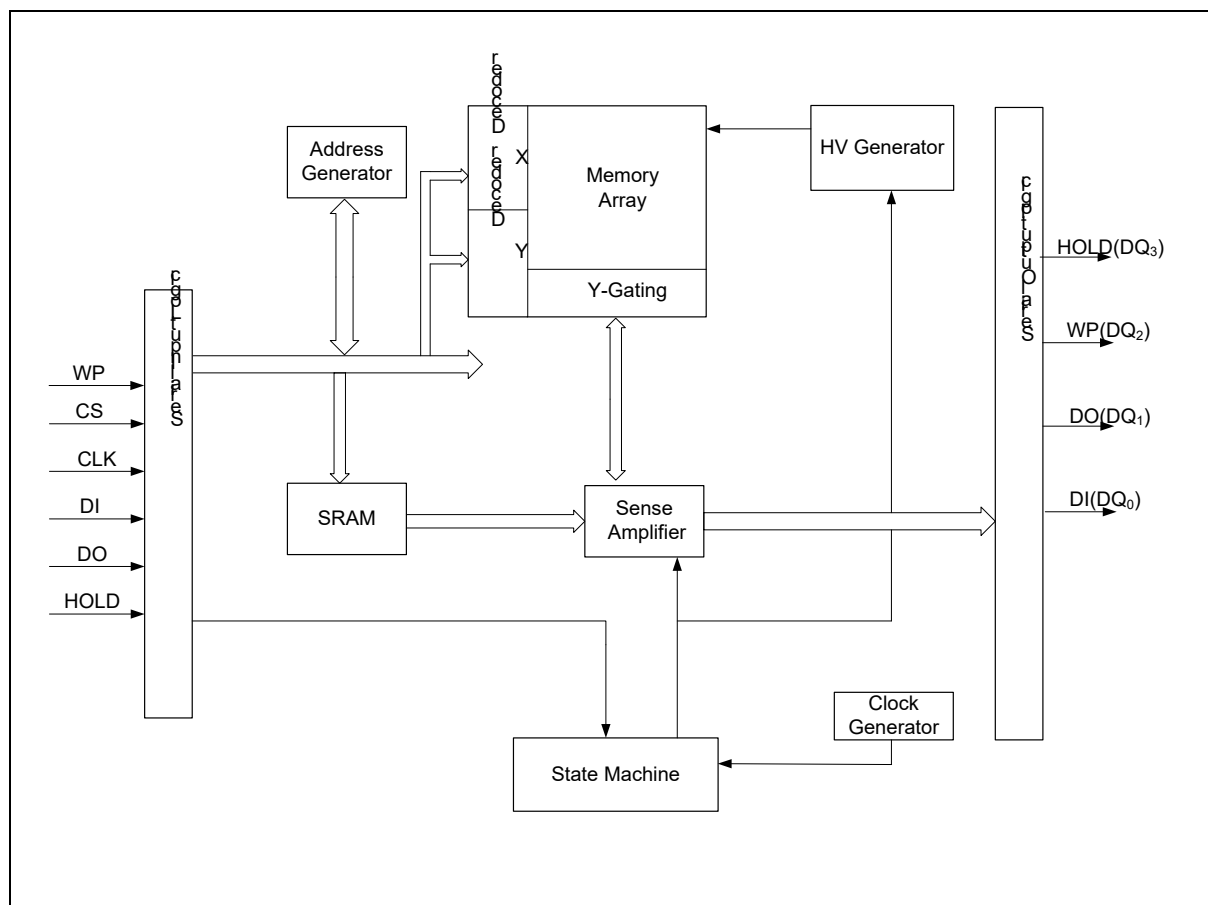
Figure 1 FM25W32AI3 Serial Flash Memory Block Diagram
