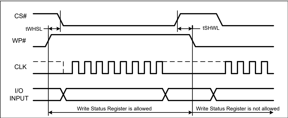
Figure 47 WP# Timing
