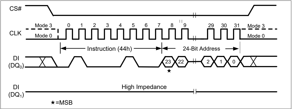
Figure 38 Erase Security Sectors Instruction (SPI Mode)
