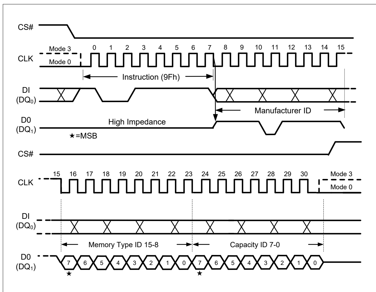
Figure 36 Read JEDEC ID Instruction (SPI Mode)
