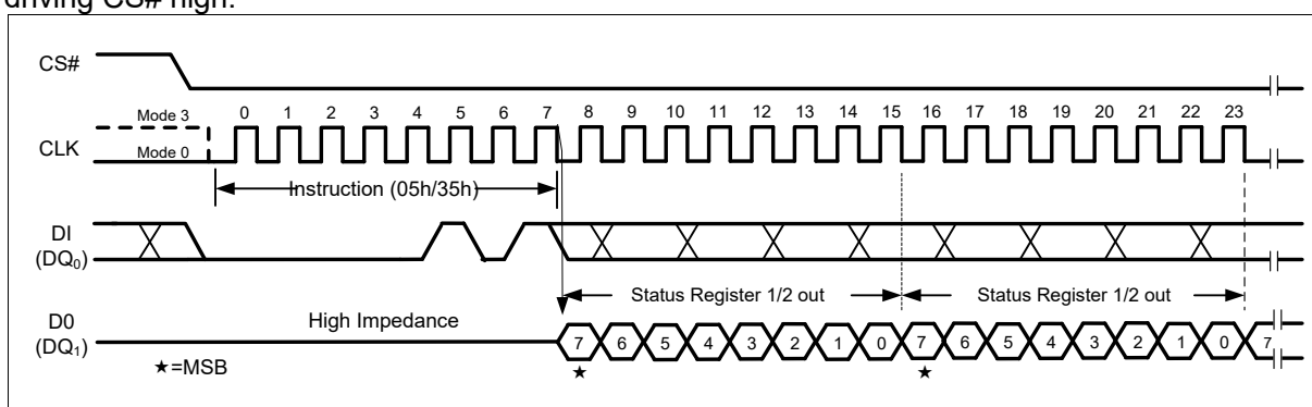
Figure 9 Read Status Register Instruction (SPI Mode)
