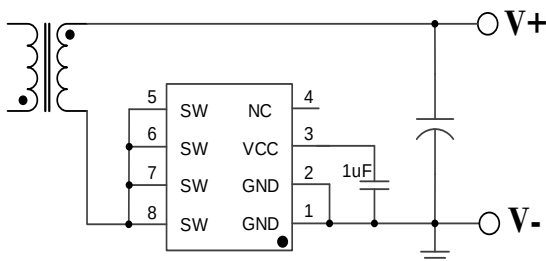
Low-side Rectification
