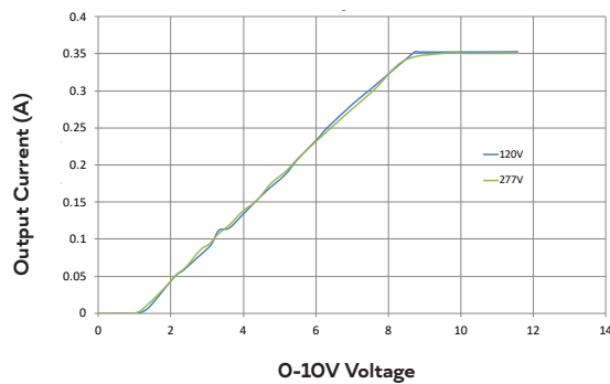
Dimming Curve
