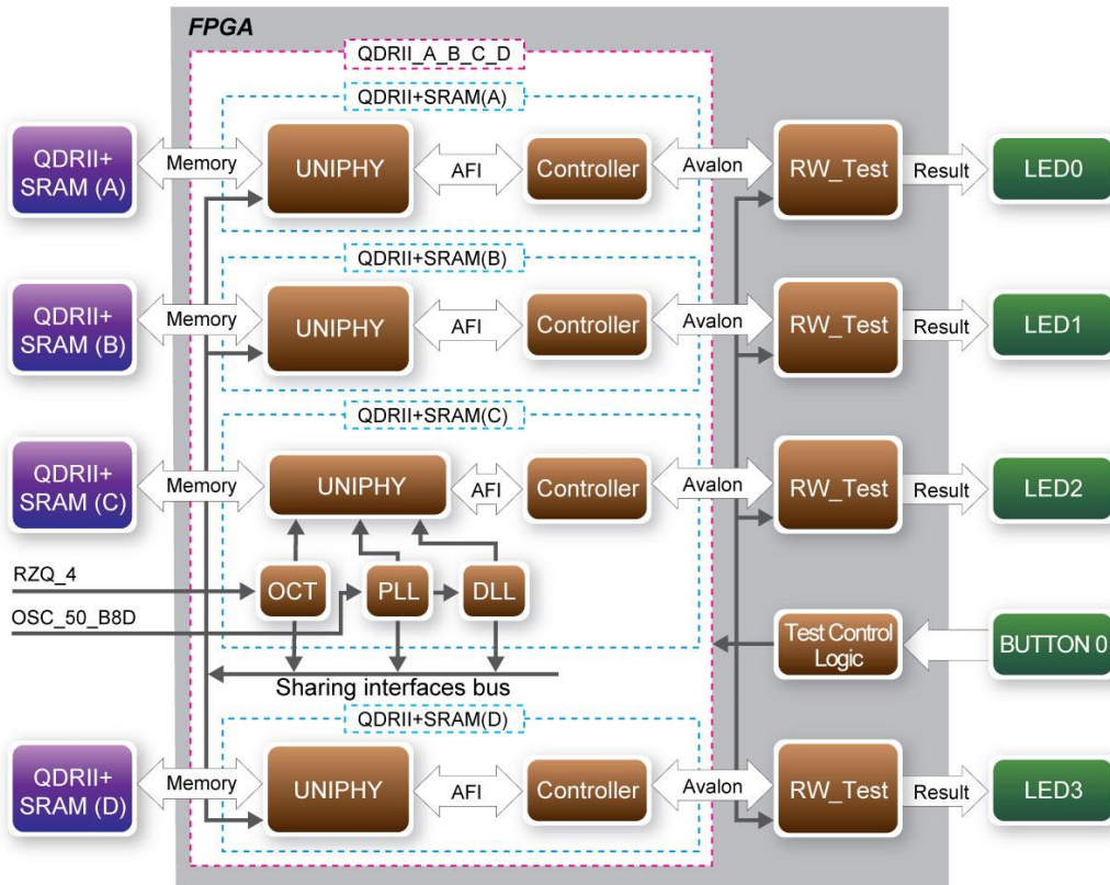
Figure 6-1 Function Block Diagram of the QDRII+ SRAM x4 Demonstration
