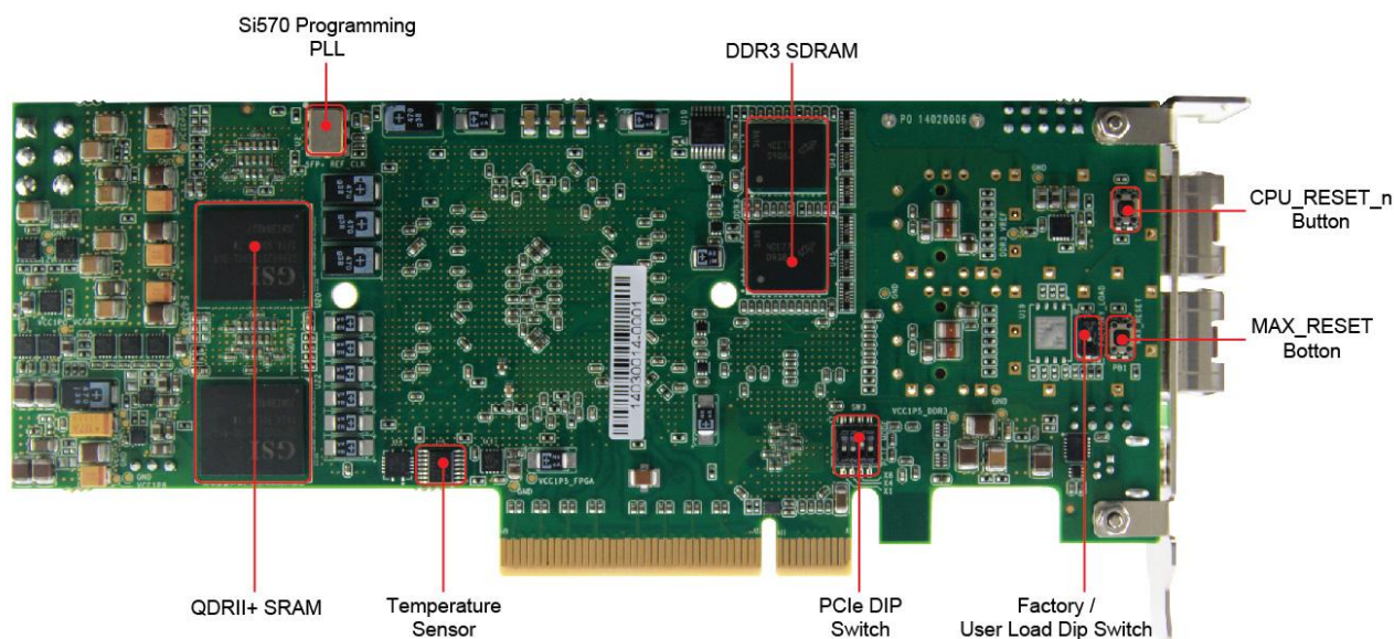
Figure 2-2 The TR5-Lite Board (Bottom)
