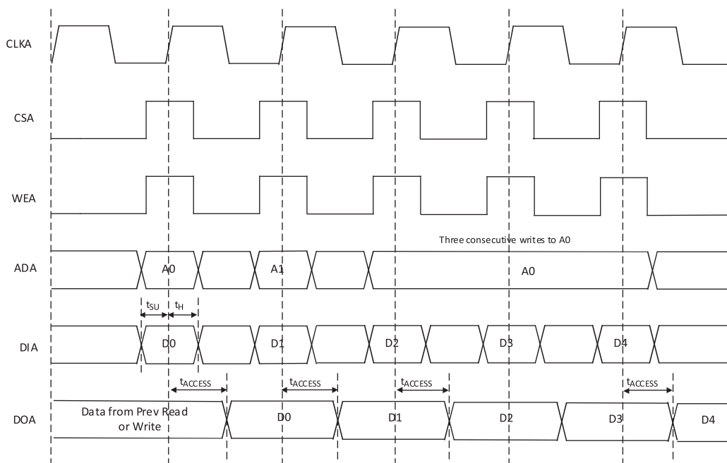
Figure 3.7. Read/Write Mode with Input and Output Registers
