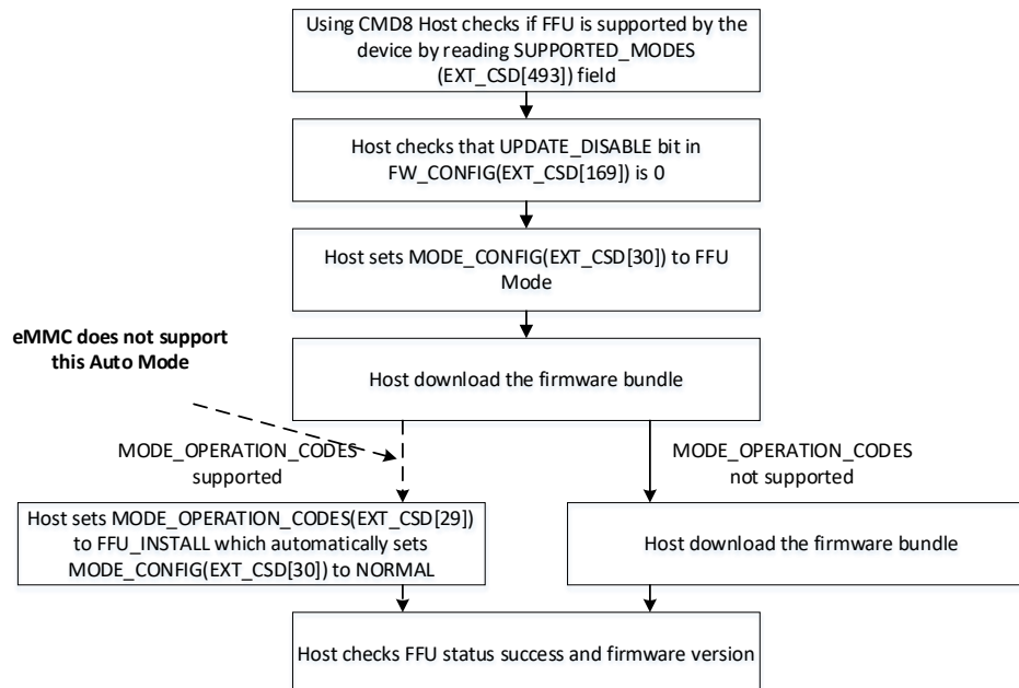
Figure 4.6-1. FFU Flow
