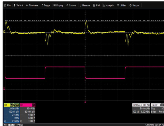
Figure 19: LCM300N Transient Response - V_O Deviation 100% to 50% load change 1A/uS slew rate V_{in} = 230V_{ac} Ch 1: V_O Ch 2: I_O
