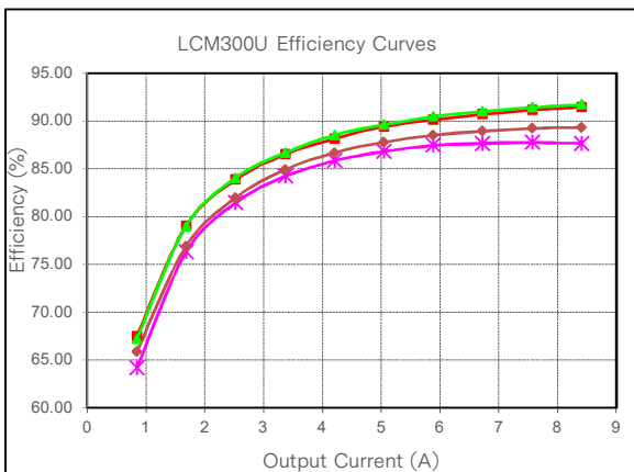
Figure 42: LCM300U Efficiency Curve @ 25°C Loading: I_{o\_main} = 10\%I_{o\_max} increment to 8.4A, I_{SB} = 0A (5V)
