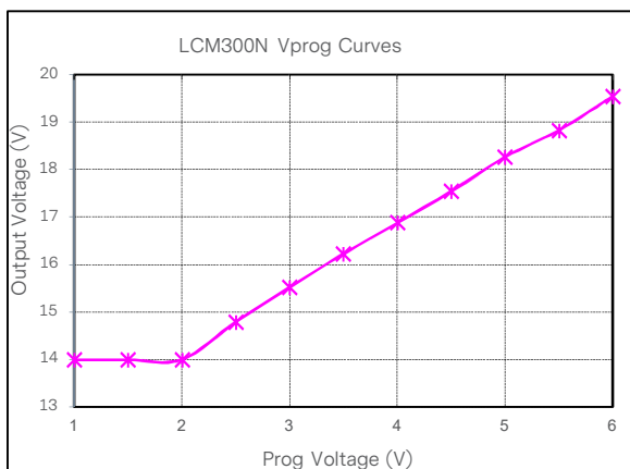
Figure 22: LCM300N Output Voltage Adjustment by V_{prog} @ 25°C — 115Vac Loading: I_O = 0A (15V), I_{SB} = 0A (5V)
