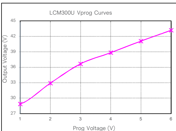
Figure 44: LCM300U Output Voltage Adjustment by Vprog @ 25°C Loading: I_o = 0A (36V), I_{SB} = 0A (5V)
