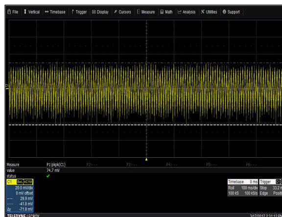
Figure 21: LCM300N Ripple and Noise Measurement V_{in} = 90V_{ac} Load: I_O = 20A (15V), I_{SB} = 2A (5V) Ch 1: V_O
