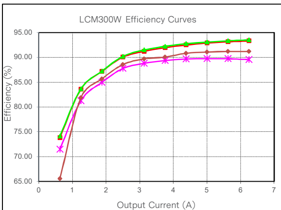
Figure 53: LCM300W Efficiency Curve @ 25°C — 90Vac — 115Vac — 230Vac — 264Vac Loading: I_{o\_main} = 10\%I_{o\_max} increment to 6.3A, I_{SB} = 0A (5V)
