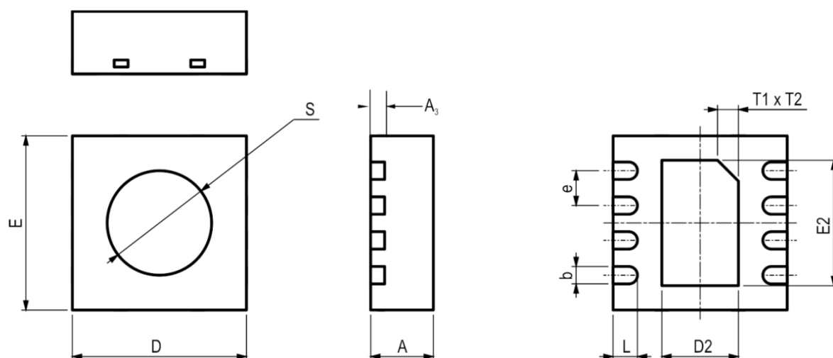
Figure 7. Dimensional drawing of GXHT30 sensor package.
