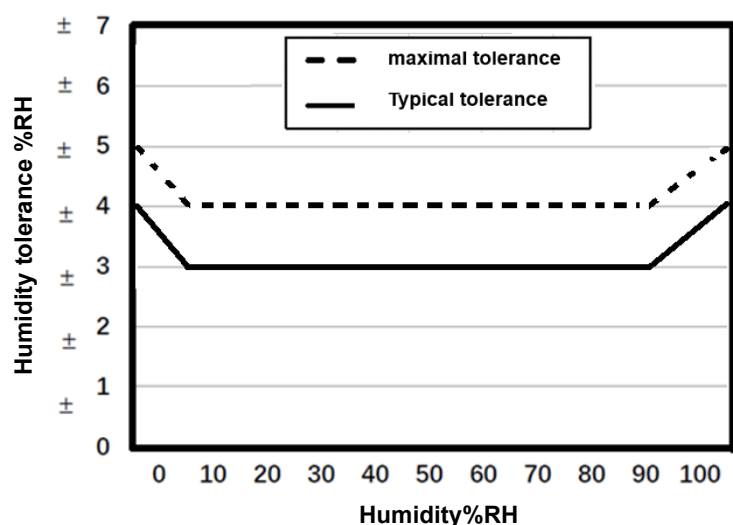
Figure 3. Tolerance of RH at 25°C for GXHT30
