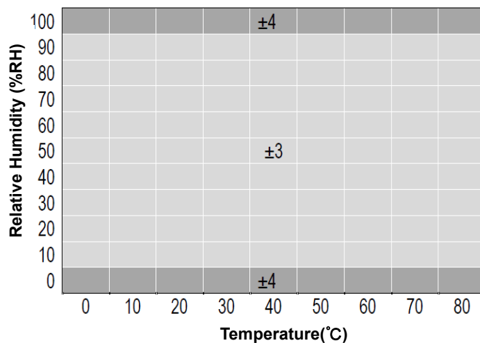
Figure 3.1 Tolerance of GXHT30 under different temperature conditions
