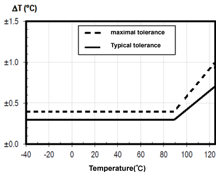
Figure 4. Temperature accuracy of GXHT30
