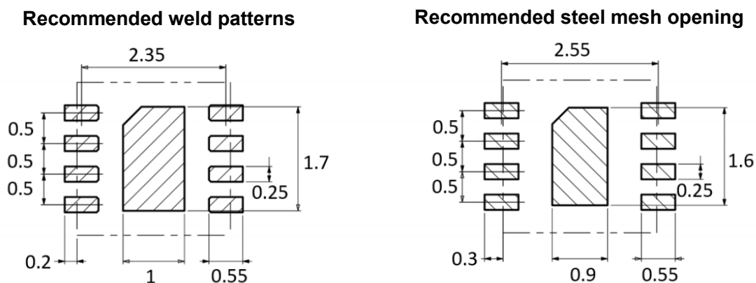
Figure 8. Recommended metal land pattern and stencil apertures for the GXHT30.
