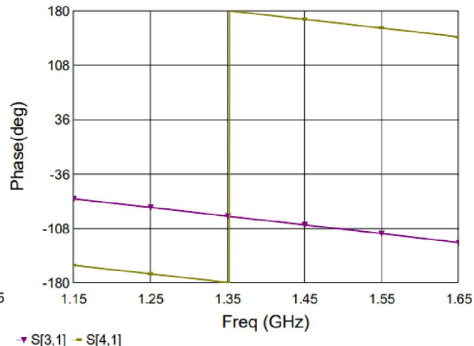
Figure 10. MHC14X03 Phase
