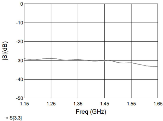
Figure 7. MHC14X03 Return Loss (S33)
