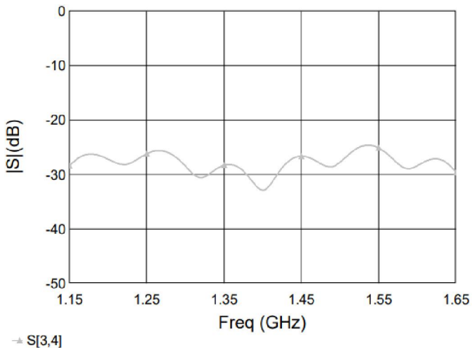
Figure 9. MHC14X03 Isolation
