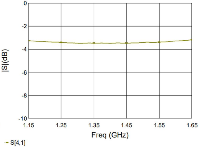
Figure 4. MHC14X03 Transmission
