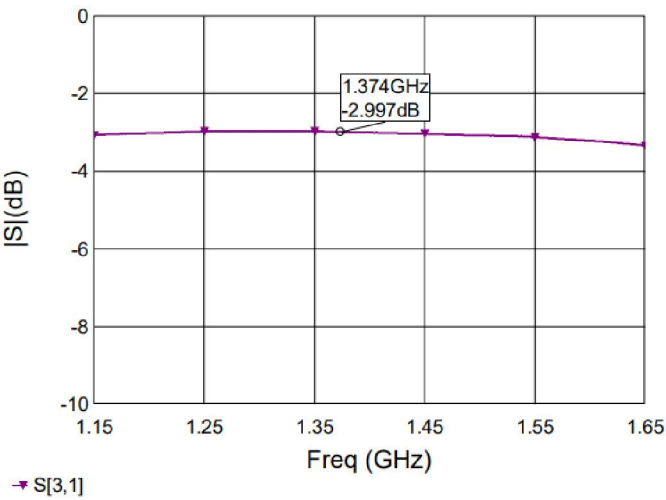
Figure 3. MHC14X03 Coupling
