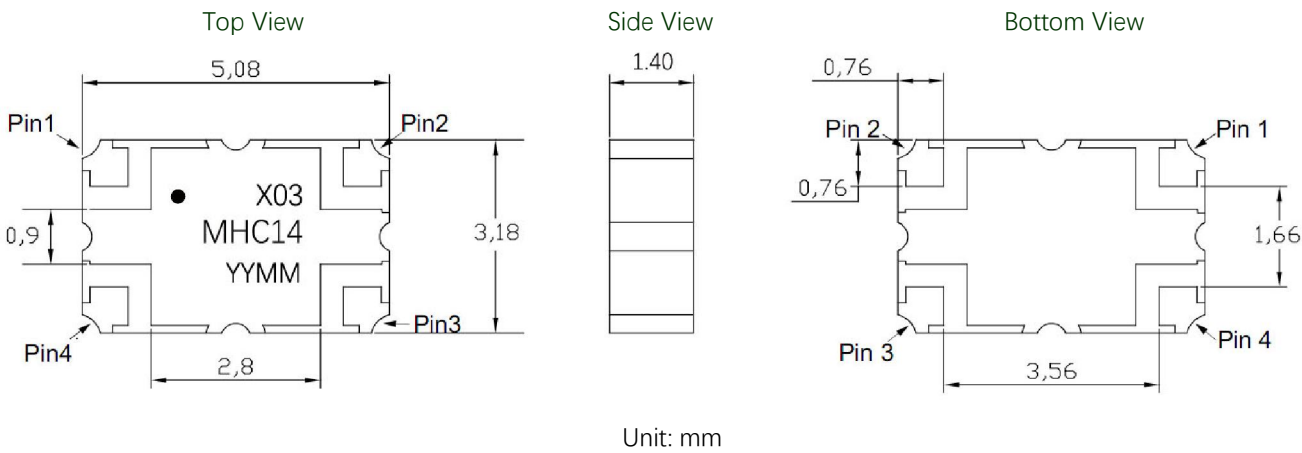
Figure 2. MHC14X03 Outline Drawing
