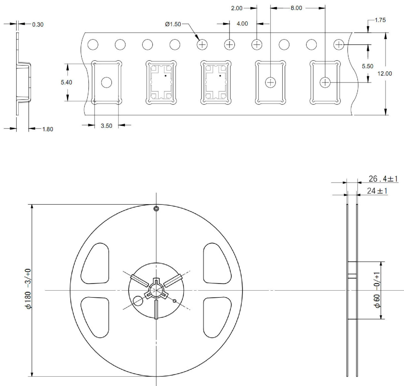
Figure 12. MHC14X03 Packaging Information
