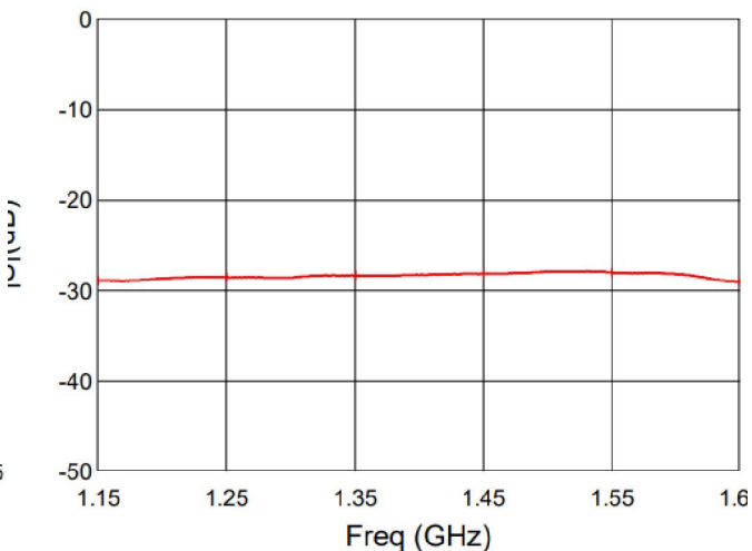
Figure 8. MHC14X03 Return Loss (S44)
