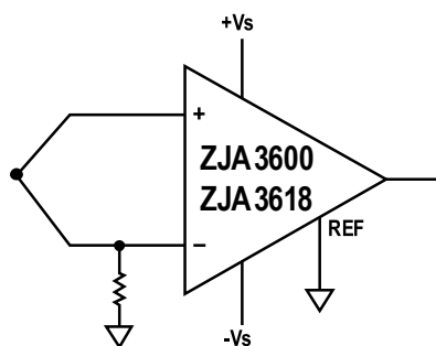
Figure 30. ZJA3600/ZJA3618 Interfaces with Thermocouple
