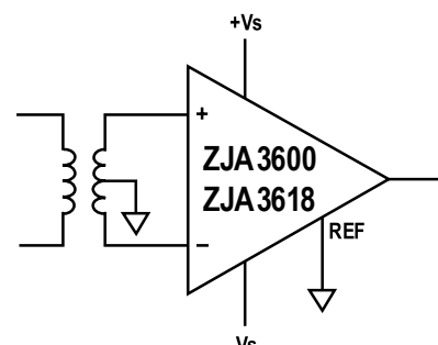
Figure 31. ZJA3600/ZJA3618 Interfaces with Transformer
