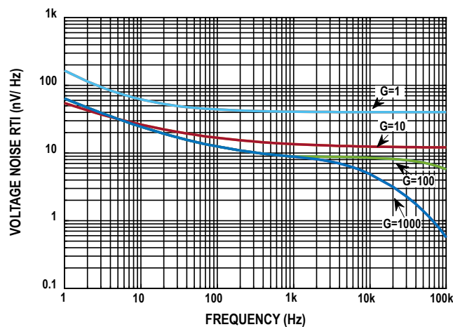
Figure 23. RTI Voltage Noise Spectral Density vs. Frequency ( G = 1 to 1000)
