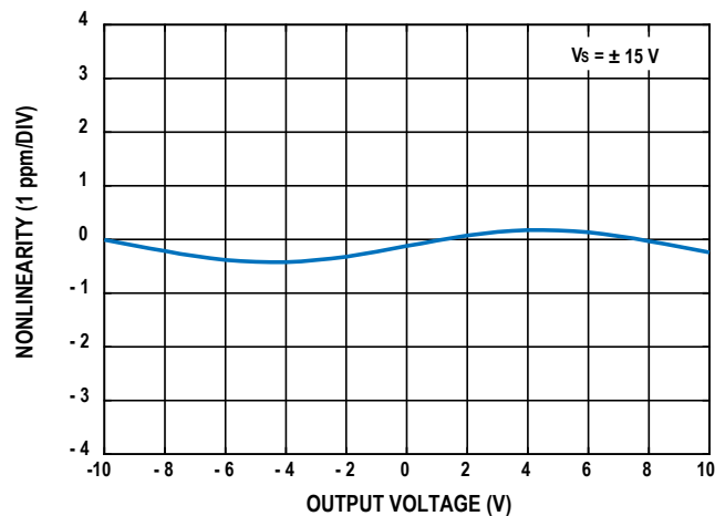
Figure 21. Gain Nonlinearity ( G = 1 , R_L = 10\text{ k}\Omega )
