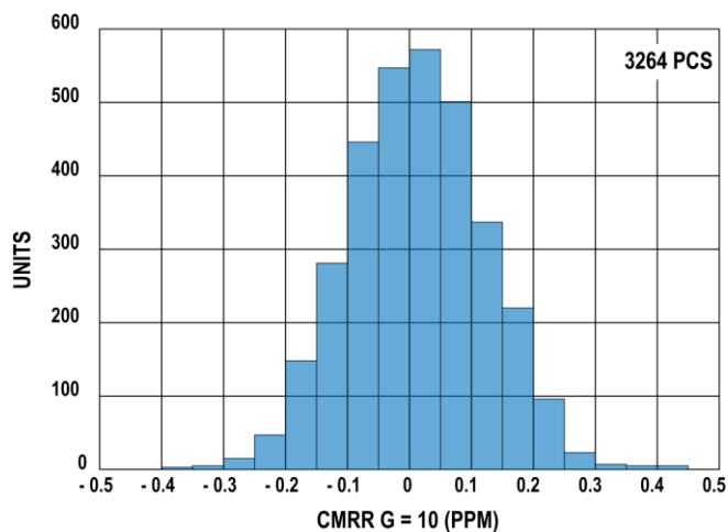
Figure 2. Typical Distribution of CMRR ( G = 10 )
