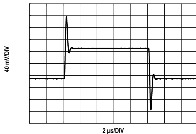
Figure 25. Small Signal Pulse Response ( G = 1 , R_L = 2\text{ k}\Omega , C_L = 100\text{ pF} )
