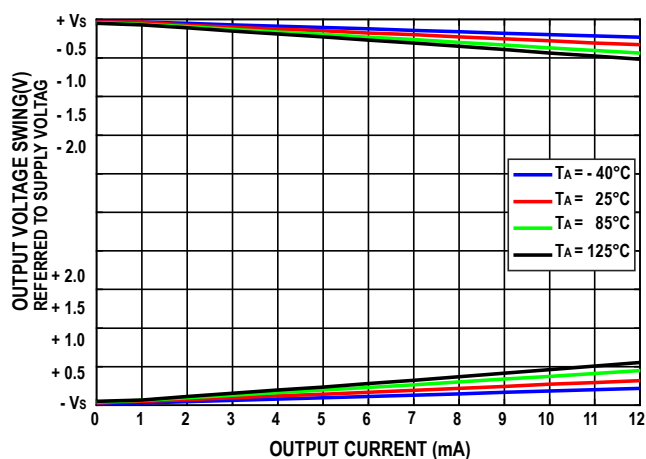
Figure 20. Output Voltage Swing vs. Output Current ( G = 1 )
