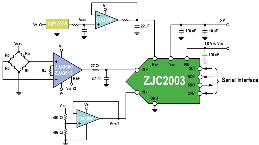
Figure 34. ZJA3600 Interfaces with Bridge Circuit
