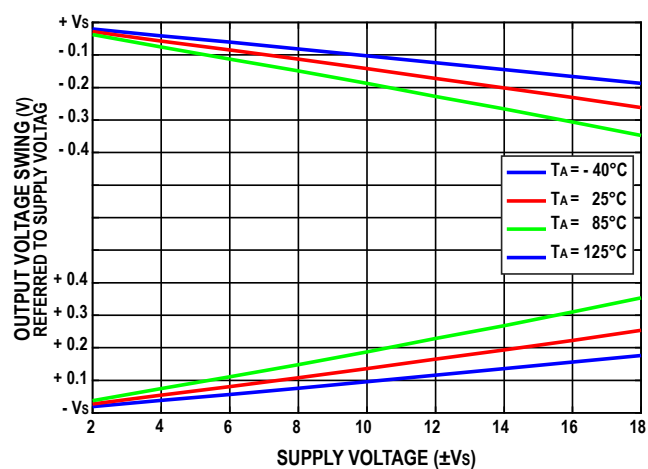
Figure 19. Output Voltage Swing vs. Supply Voltage (G = 1, R_L = 2\text{ k}\Omega )
