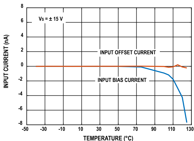
Figure 8. . Input Bias Current &amp; Offset Current vs. Temperature
