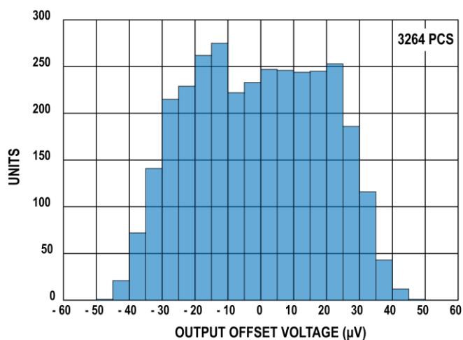
Figure 4. Typical Distribution of Output Offset Voltage V_{OSO}
