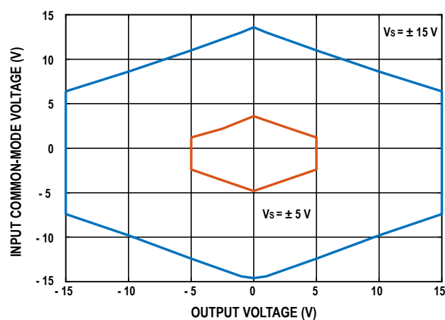
Figure 9. Input Common-Mode Voltage vs. Output Voltage (G = 1)
