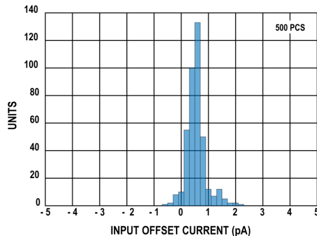
Figure 7. Typical Distribution of Input Offset Current
