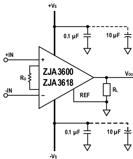
Figure 33. Supply Decoupling, REF, and Output Referred to Local Ground
