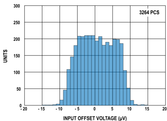
Figure 3. Typical Distribution of Input Offset Voltage V_{OSI}
