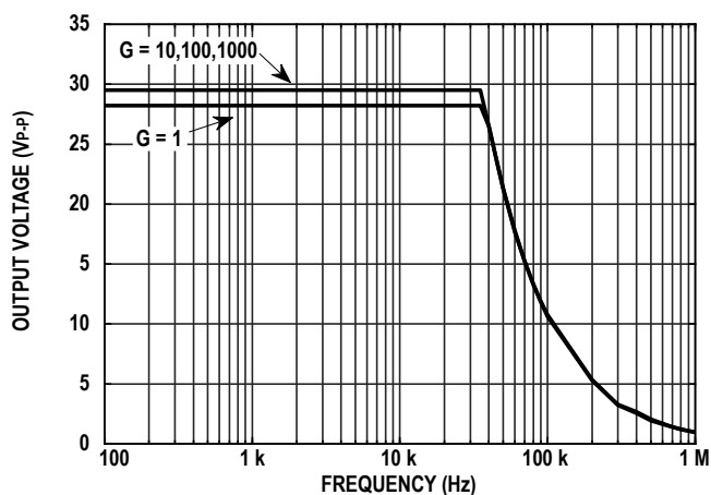
Figure 24. Large Signal Frequency Response
