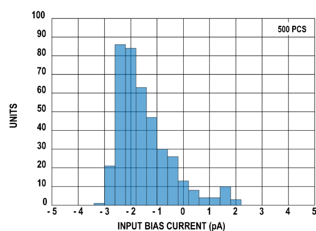
Figure 5. Typical Distribution of Input Bias Current I_{BIAS}
