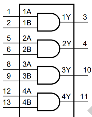
Figure 1. Functional diagram
