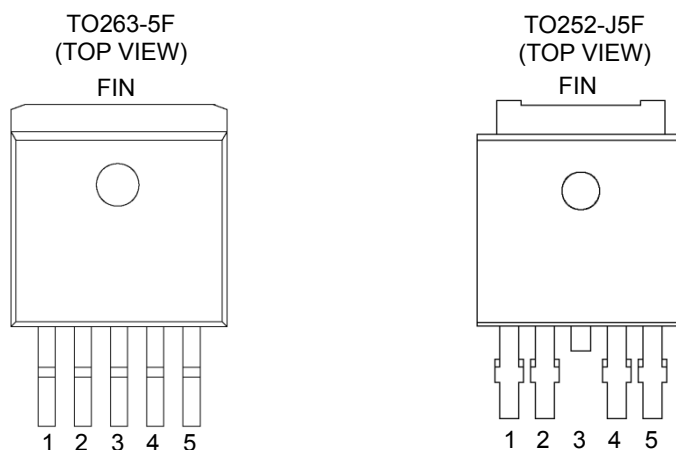
Figure 3. Pin configurations
