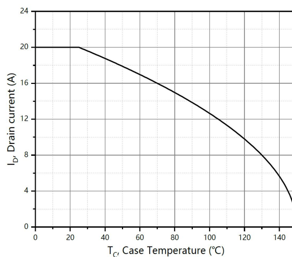
Drain current
