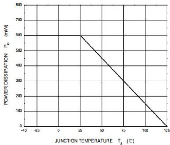
Figure 6: Power Characteristics
