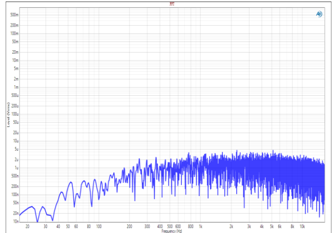
Fig 14-Noise Floor ( R_L=8\Omega )
