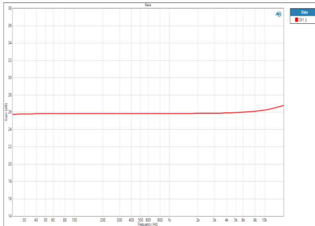
Fig 13-Frequency Response
