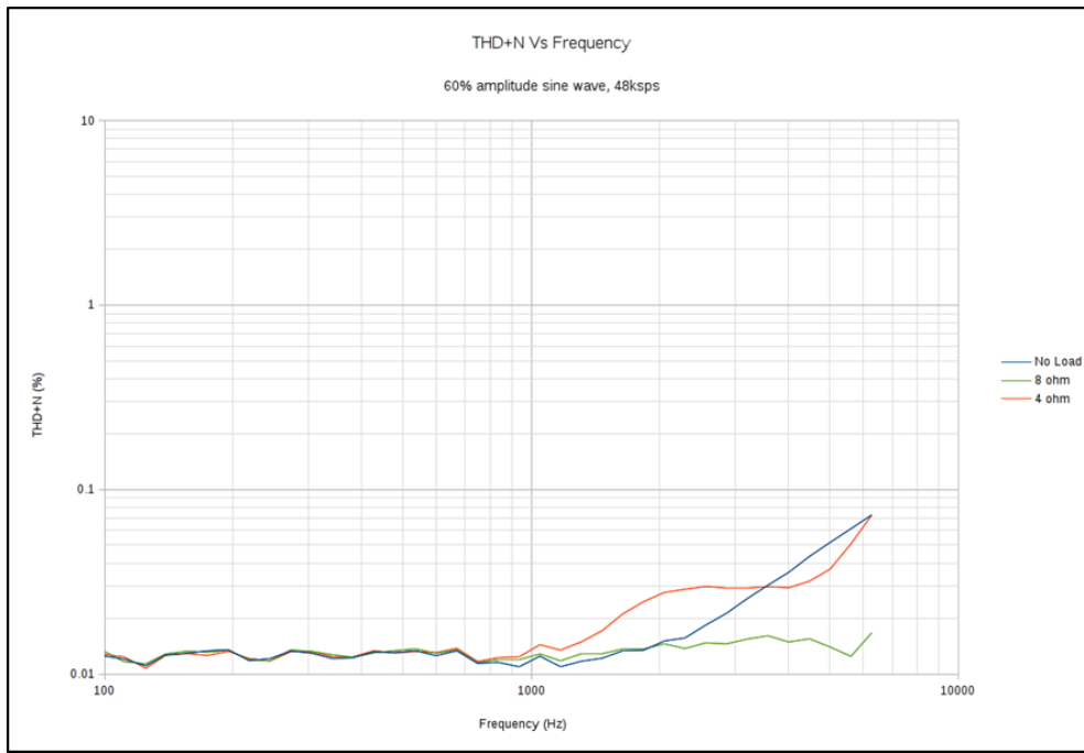
Figure 49 Class D amplifier THD+N vs. Frequency 48kps
