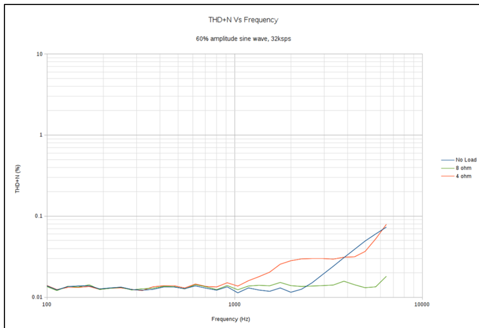
Figure 50 Class D amplifier THD+N vs. Frequency 32kps
