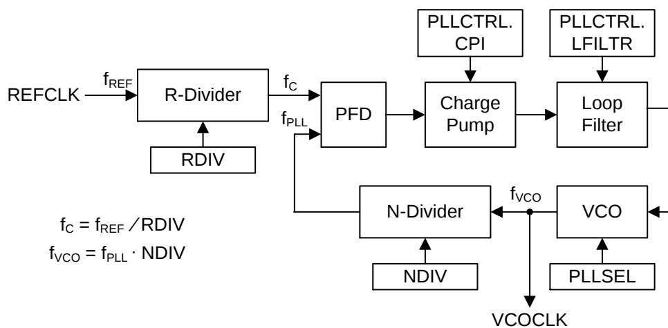
Figure 9 Integer-N PLL
