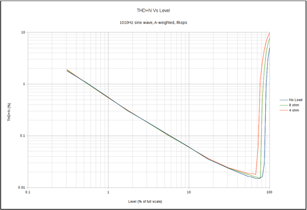
Figure 47 Class D amplifier THD+N vs. Level 8ksps
