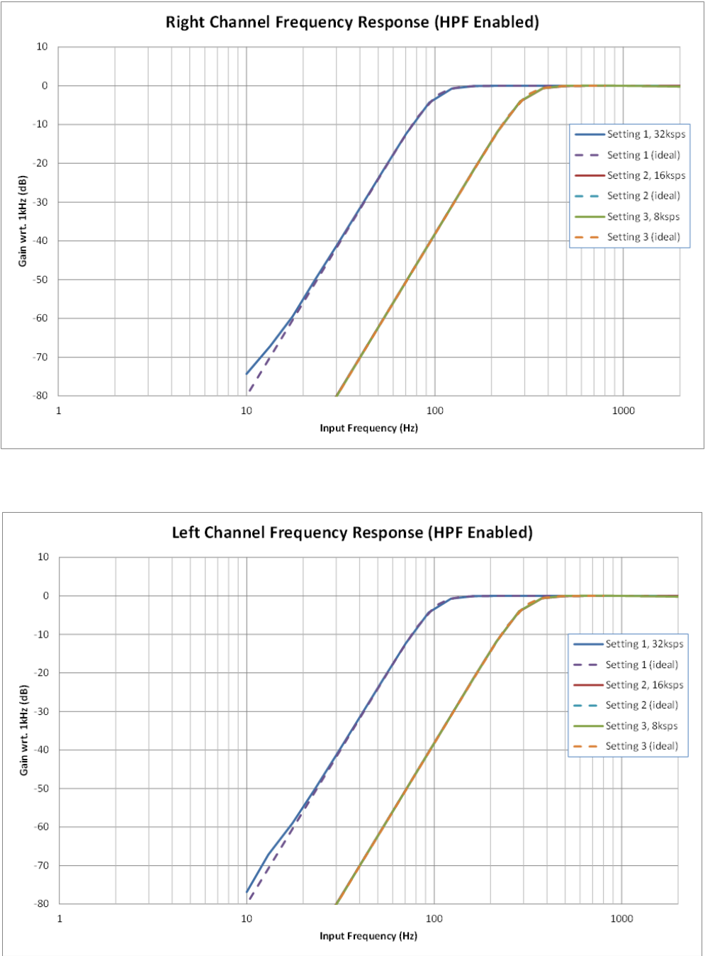
Figure 59 High Pass Filter Response Microphone Channels
