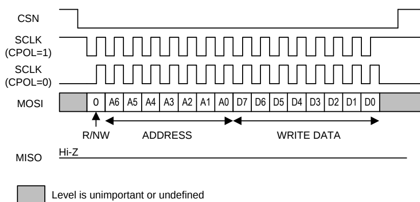
Figure 25 SPI Write Transfer
