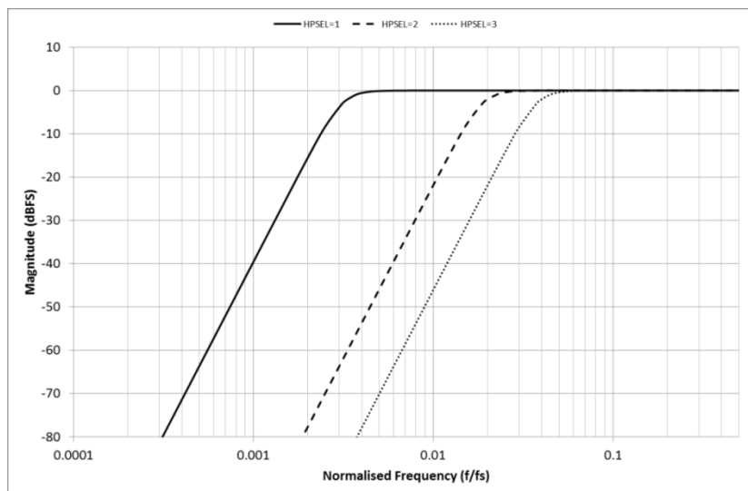
Figure 23 High Pass Filter Frequency Response
