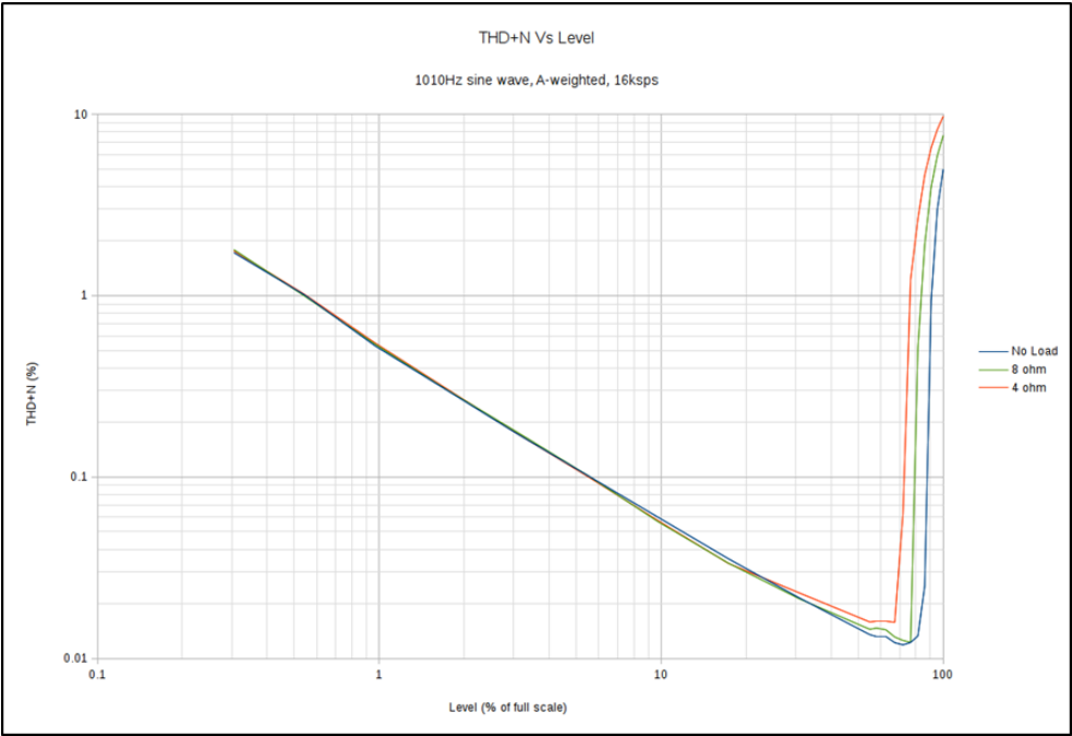
Figure 46 Class D amplifier THD+N vs. Level 16ksps
