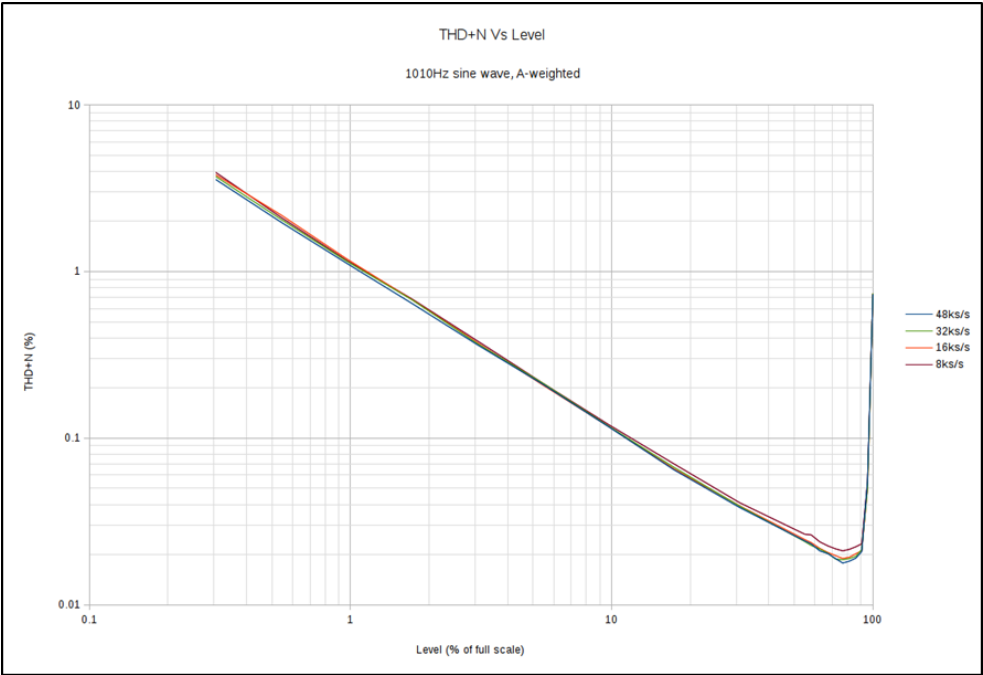
Figure 48 Line out amplifier THD+N vs. Level 48/32/16/8ksps
