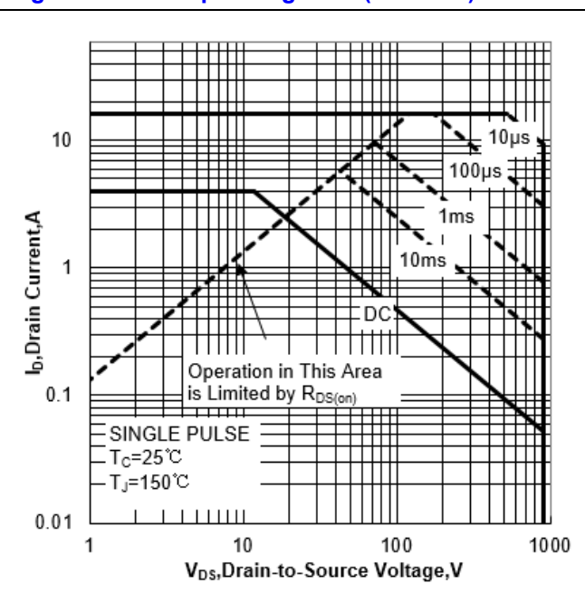
Figure 1b Safe Operating Area (TO-220F)
