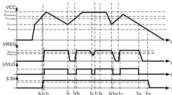
Figure 8: Operation Waveform of External Supply Mode
