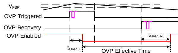
Figure 16: Output OVP
