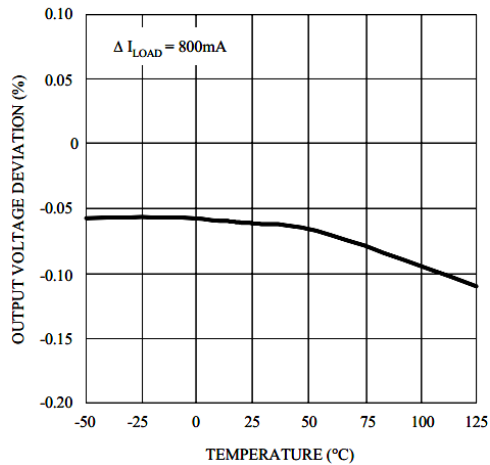
Load Regulation
