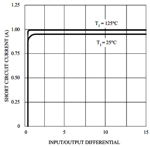
Short-Circuit Current
