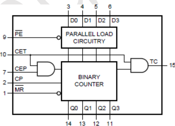
Figure 3. Functional diagram
