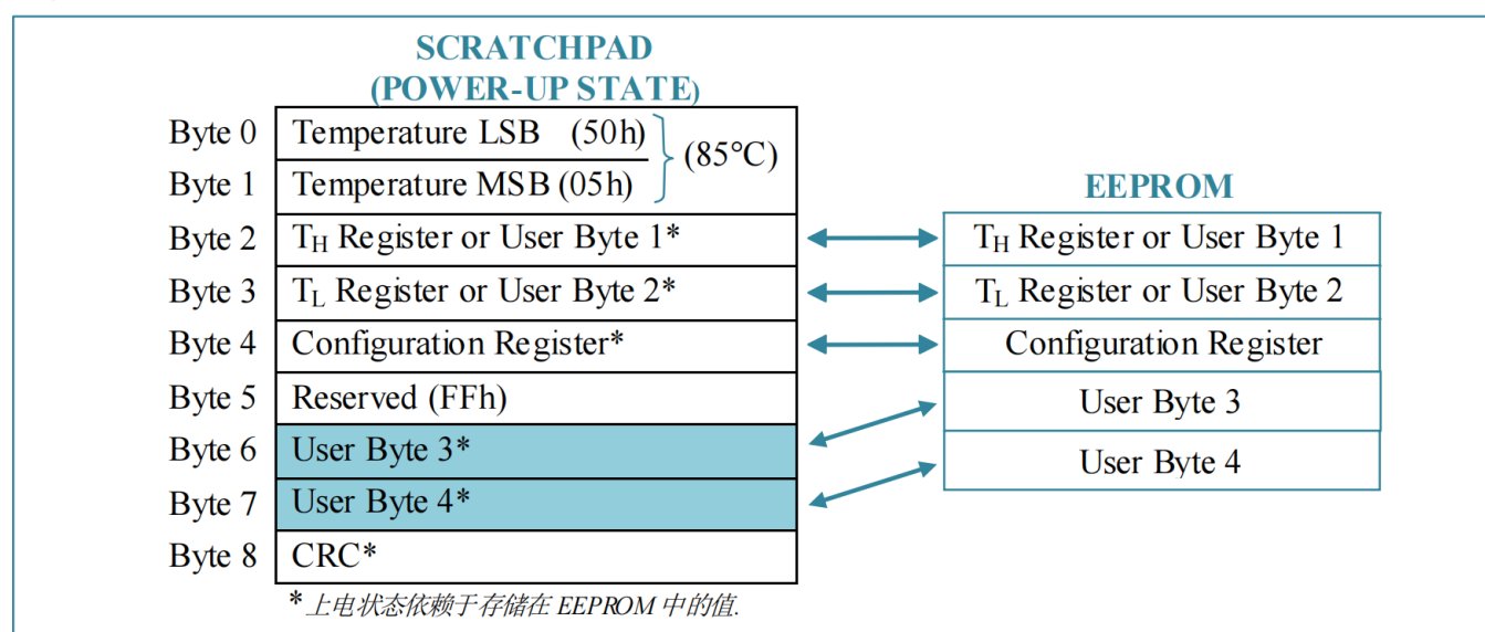
Figure7. GX1820 Memory Map
