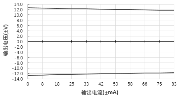
输出电压Vs输出电流(Vin=5V)@E0512S-2WR2
