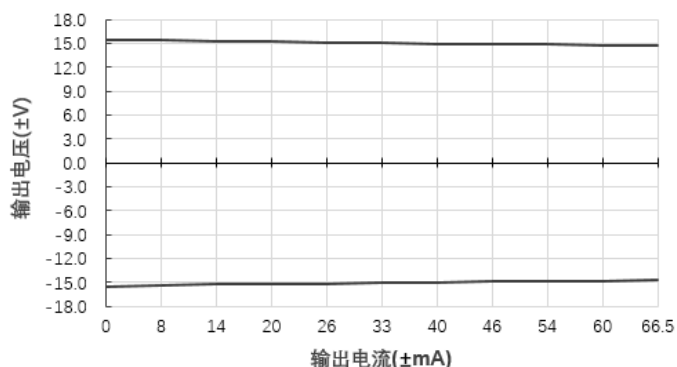
输出电压Vs输出电流(Vin=12V)@E1215S-2WR2
