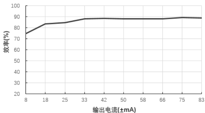
效率Vs输出电流(Vin=24V)@E2412S-2WR2
