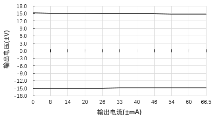
输出电压Vs输出电流(Vin=24V)@E2415S-2WR2
