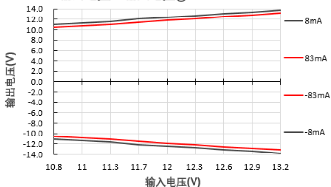
输出电压Vs输入电压@E1212S-2WR2
