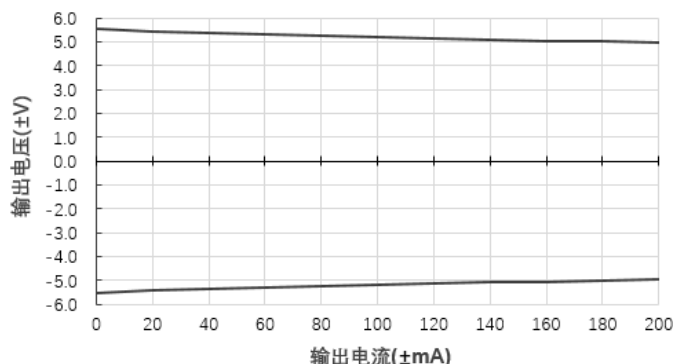
输出电压Vs输出电流(Vin=12V)@E1205S-2WR2
