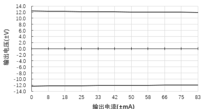
输出电压Vs输出电流(Vin=24V)@E2412S-2WR2
