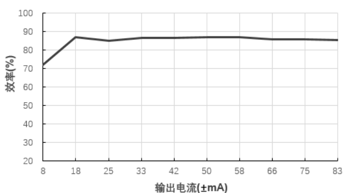
效率Vs输出电流(Vin=5V)@E0512S-2WR2
