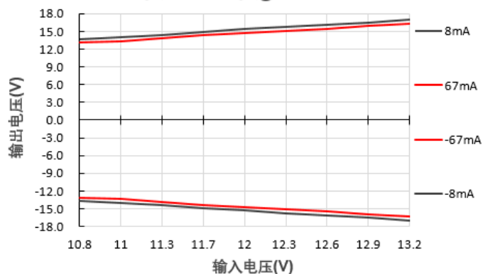
输出电压Vs输入电压@E1215S-2WR2
