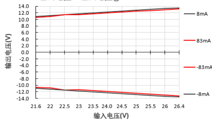
输出电压Vs输入电压@E2412S-2WR2
