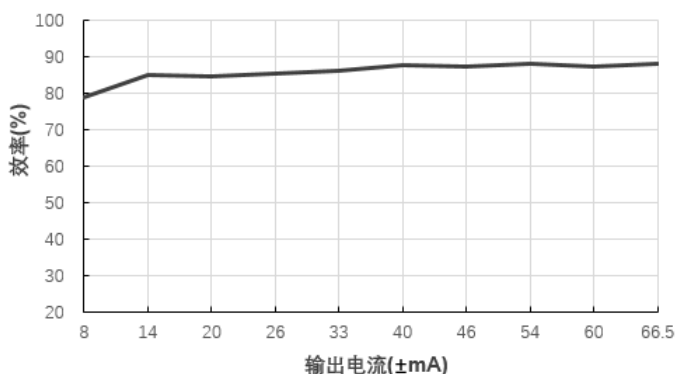
效率Vs输出电流(Vin=12V)@E1215S-2WR2
