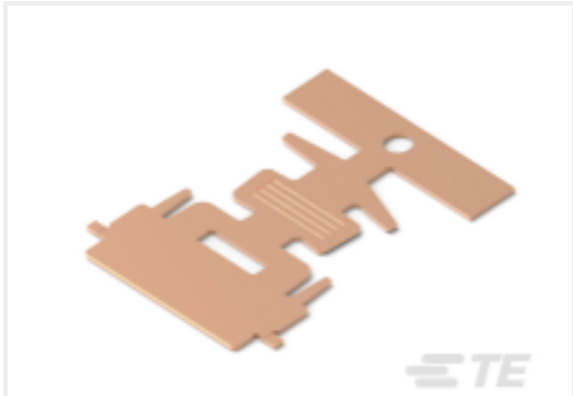
TE Part #1-1600961-7 CONT 12-16 AWG PWR, MFBL PLATE
