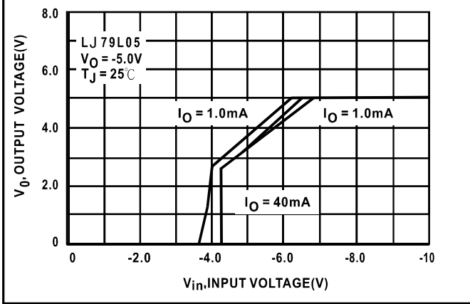
Figure 1. Dropout Characteristics
