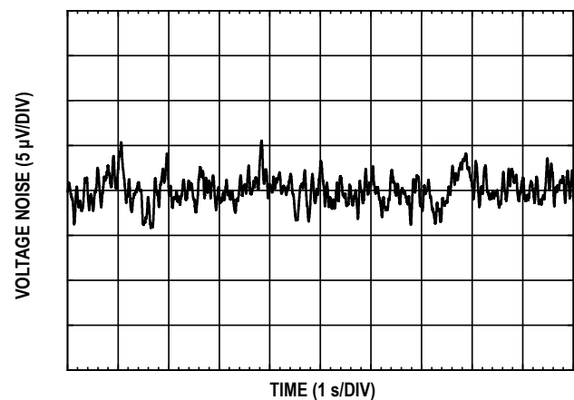
Figure 8. ZJR1004-5 0.1~10 Hz Noise
