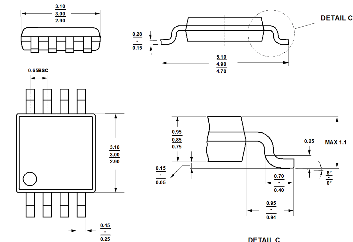
Figure 24. 8-Lead MSOP Package Dimensions shown in millimeters
