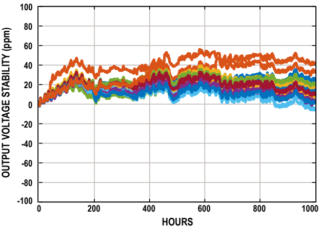
Figure 16. Long-Term Stability (SOIC-8 package)
