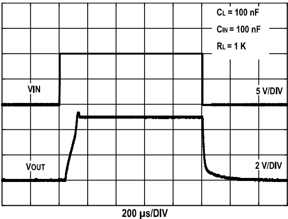
Figure 10. Power-On/Off Response
