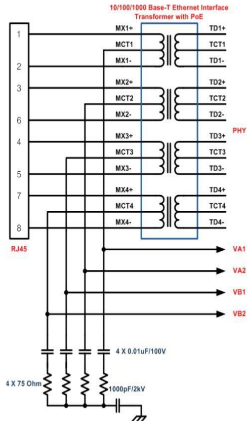
Figure 2: Typical System Diagram
