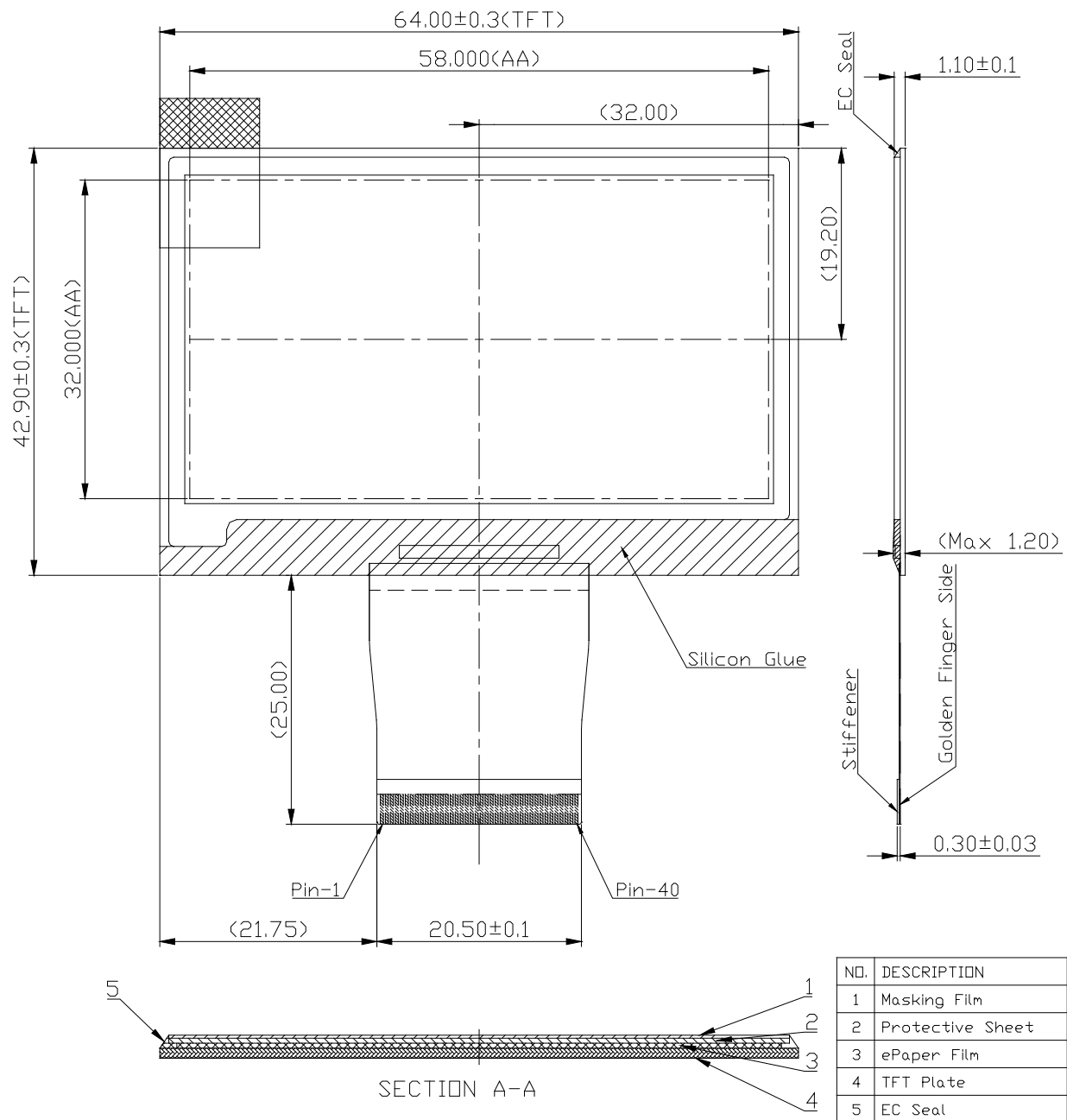
Figure 1-1 EPD Drawing
