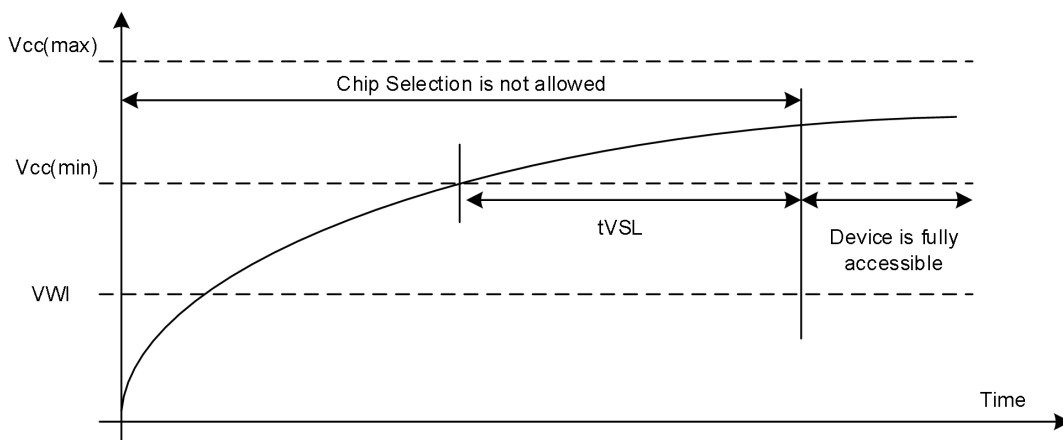
Figure27. Power-On Timing
