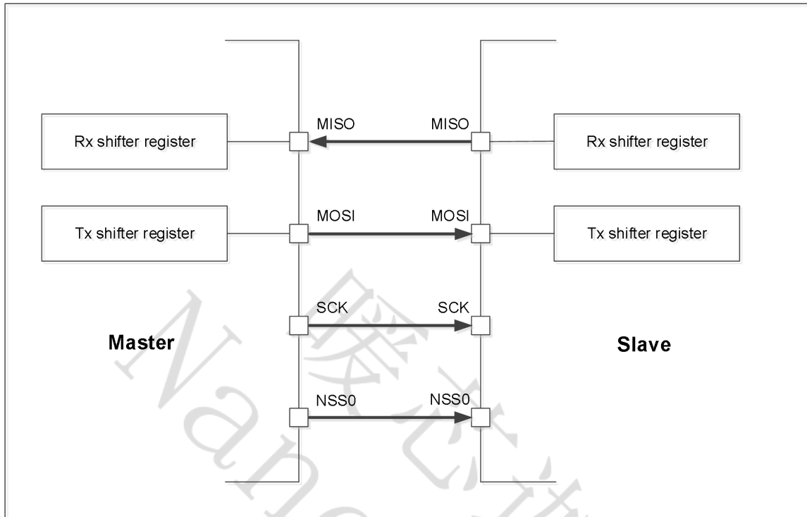
Figure 7 Full-duplex Application
