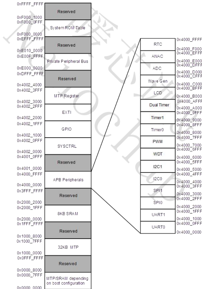
Figure 2 Memory Map Diagram
