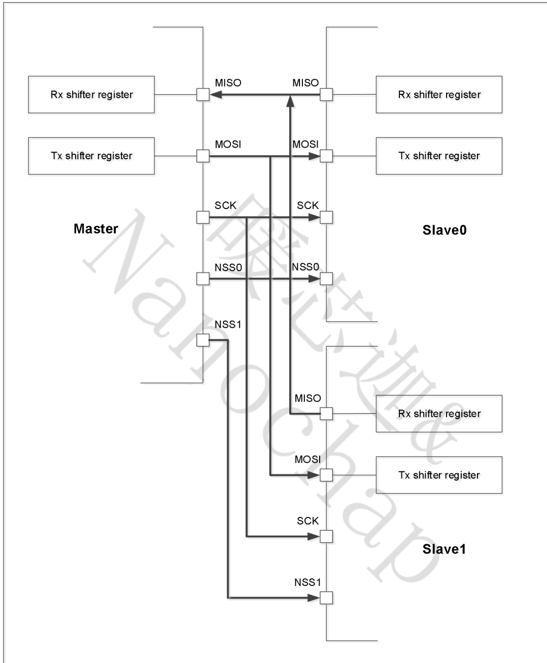
Figure 11 Multi-slave Application
