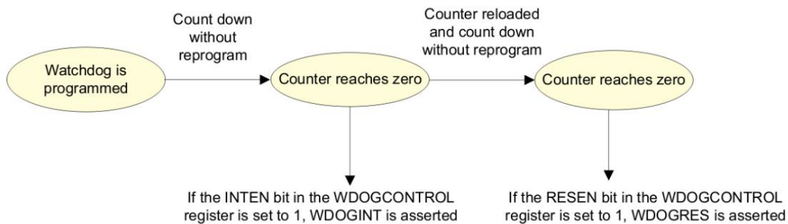
Figure 19 WDT Flow Diagram
