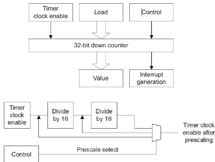
Figure 22 Dual-Timers Block Diagram
