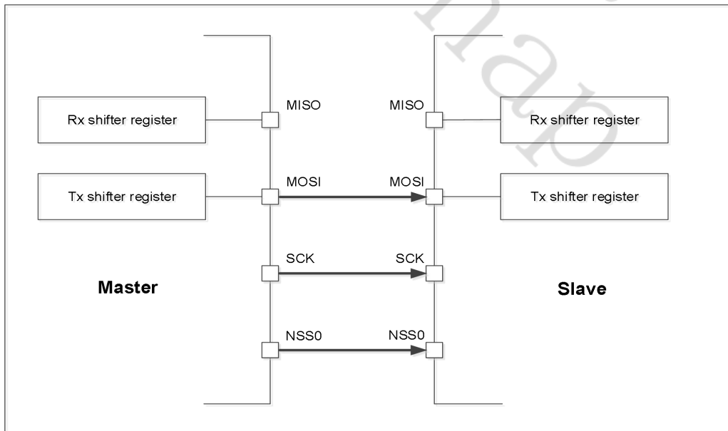
Figure 9 Master in Transmit-only and Slave in Receive-only Mode
