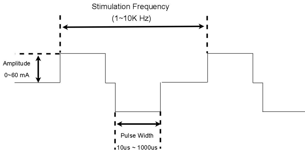
Figure 25 Square waveform
