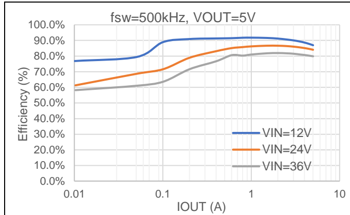
Figure 1 Power Efficiency
