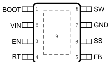
Top View: GBI1430/1432 eSOP-8L
