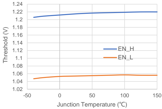
Figure 7 Enable Threshold
