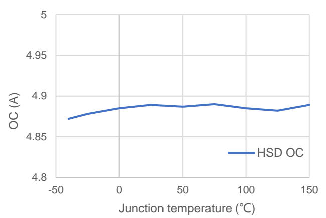
Figure 8 Over Current
