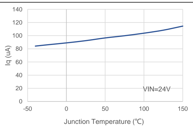
Figure 6 Quiescent Current
