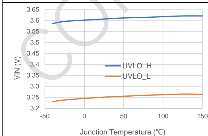
Figure 5 V_{IN} UVLO Threshold
