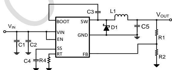
Simplified Schematic
