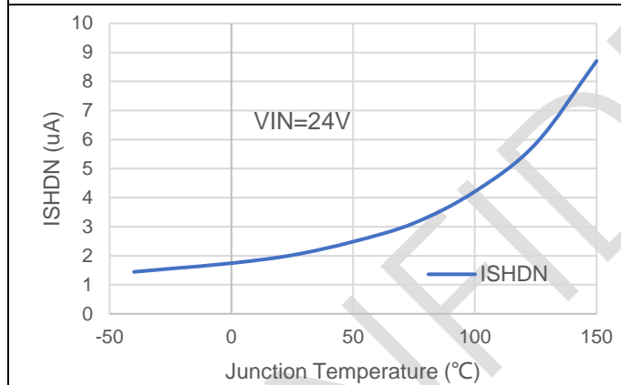
Figure 3 Shutdown Current
