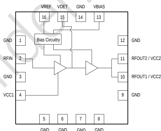
Figure 2. GSM0520 Function Block Diagram
