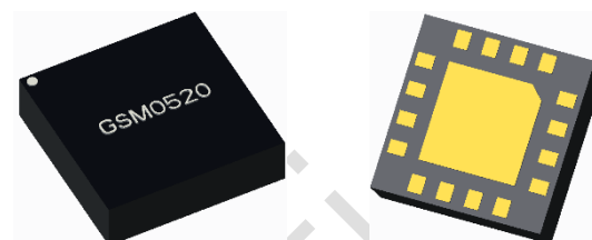
Figure 1. 16 Pad 3 x 3 mm Laminate Package
