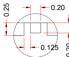
LEAD DETAIL
