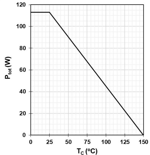
Figure 16 Power dissipation
