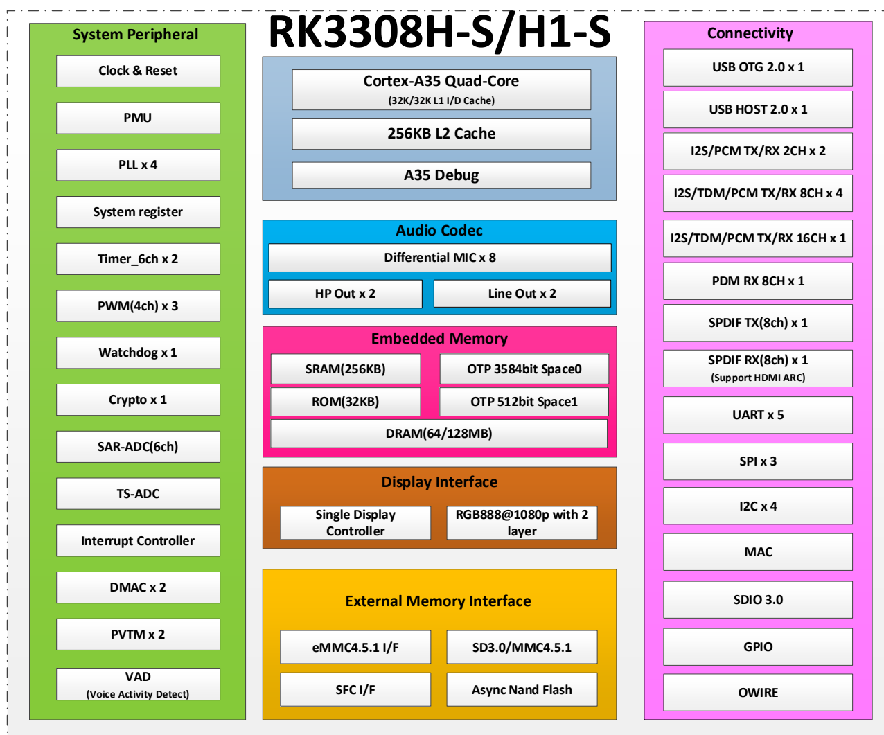
Fig.1-2 RK3308H-S/RK3308H1-S Block Diagram
