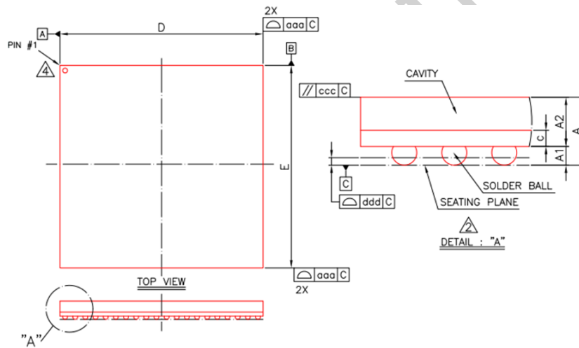
Fig.2-4 RK3308B-S Package Top View and Side View
