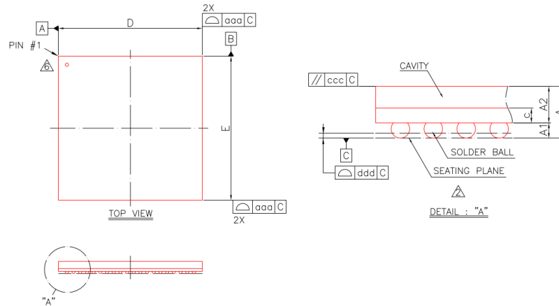
Fig.2-7 RK3308H-S/RK3308H1-S Package Top View and Side View
