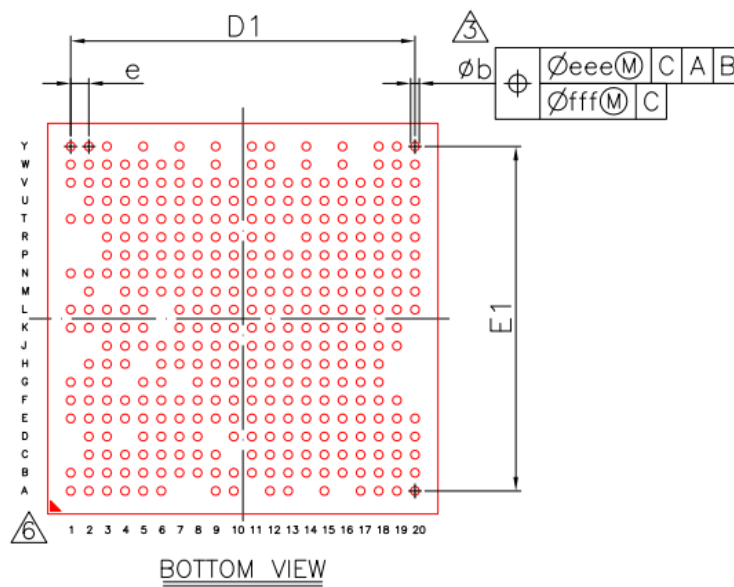
Fig.2-8 RK3308H-S/RK3308H1-S Package bottom view
