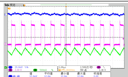
Fig. 9 Steady State Waveform
