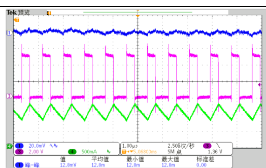
Fig. 14 Steady State Waveform
