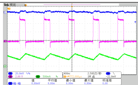
Fig. 6 Steady State Waveform
