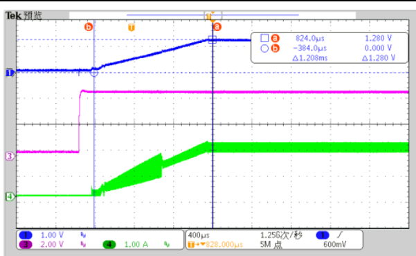
Fig. 39 VIN Power On/Off, I_{OUT} = 0.5\text{A} Power On
