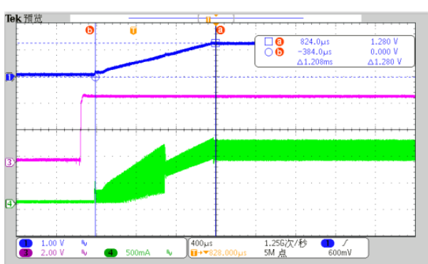
Fig. 37 VIN Power On/Off, I_{OUT} = 0\text{A} Power On
