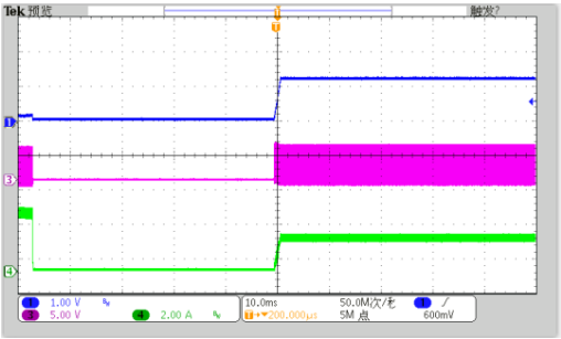
Fig. 50 Short Recovery
