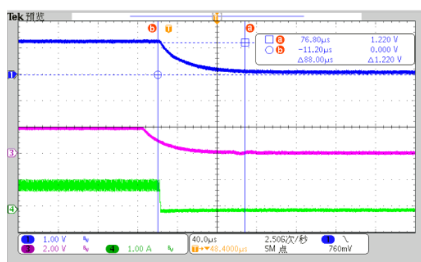
V IN = 5V, V OUT = 1.2V, C IN =10uF Fig. 46 EN Power On/Off, I OUT = 1A Power Off
