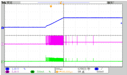
Fig. 50 Short Recovery
