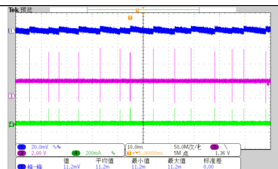
Fig. 9 Steady State Waveform
