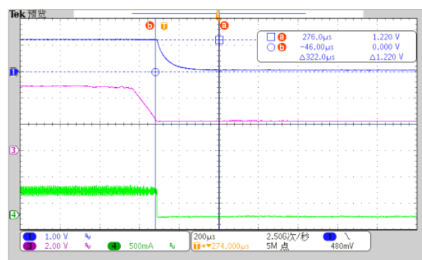
Fig. 38 VIN Power On/Off, I_{OUT} = 0\text{A} Power Off
