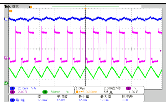
Fig. 10 Steady State Waveform
