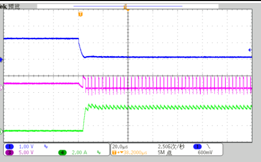
Fig. 53 Short
