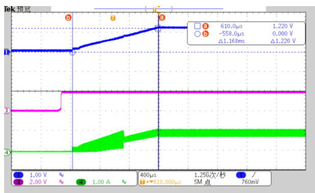
V IN = 5V, V OUT = 1.2V, C IN =10uF Fig. 45 EN Power On/Off, I OUT = 1A Power On
