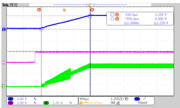
V IN = 5V, V OUT = 1.2V, C IN =10uF Fig. 47 EN Power On/Off, I OUT = 2A Power On
