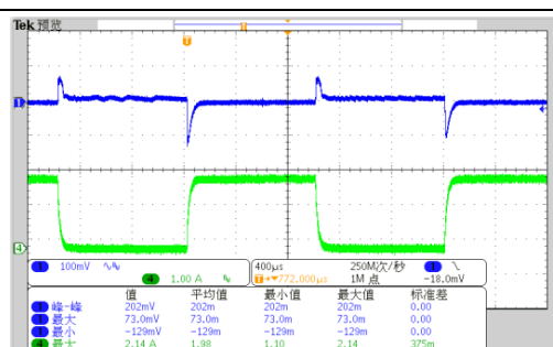
Fig. 22 Transient Waveform
