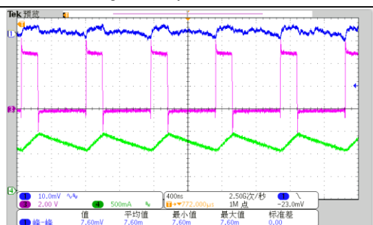
Fig. 5 Steady State Waveform
