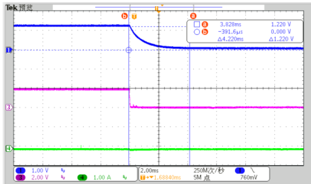
V IN = 5V, V OUT = 1.2V, C IN =10uF Fig. 44 EN Power On/Off, I OUT = 0A Power Off
