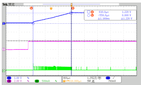
V IN = 5V, V OUT = 1.2V, C IN =10uF Fig. 43 EN Power On/Off, I OUT = 0A Power On
