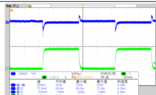
Fig. 26 Transient Waveform
