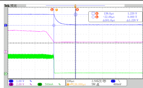
Fig. 40 VIN Power On/Off, I_{OUT} = 0.5\text{A} Power Off
