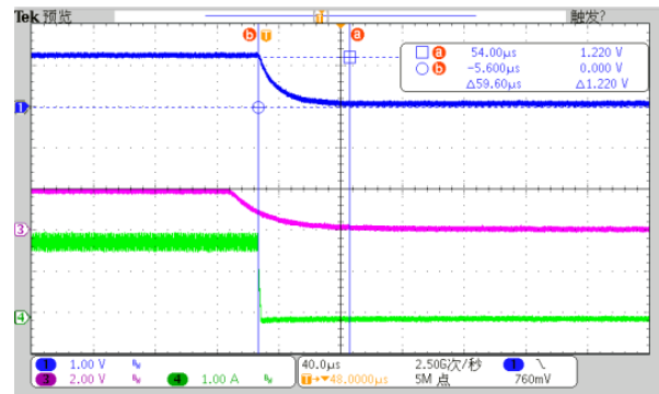
V IN = 5V, V OUT = 1.2V, C IN =10uF Fig. 48 EN Power On/Off, I OUT = 2A Power Off
