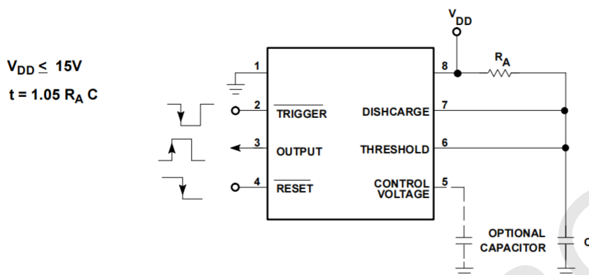
Figure 1: Monostable
