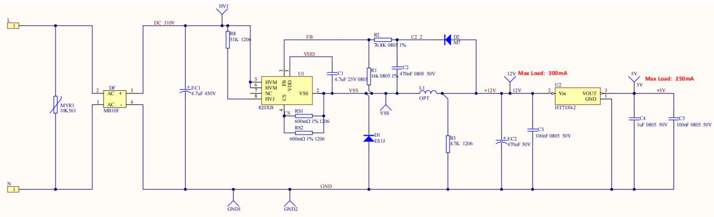
Figure 4. SS8201B Typical Application Circuit
