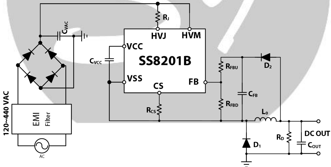
Figure 1. SS8201B Typical Application Circuit
