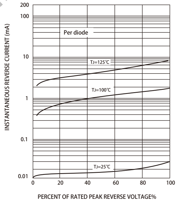
FIG. 4-TYPICAL REVERSE CHARACTERISTICS
