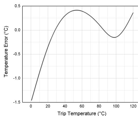
Temperature Error vs Trip Temperature
