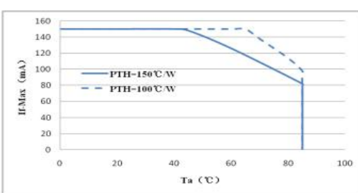
图 6 最大驱动电流与室温曲线 Maximum Driving Forward DC Current vs. Ambient Temperature (Derating based on Tj max=125°C)
