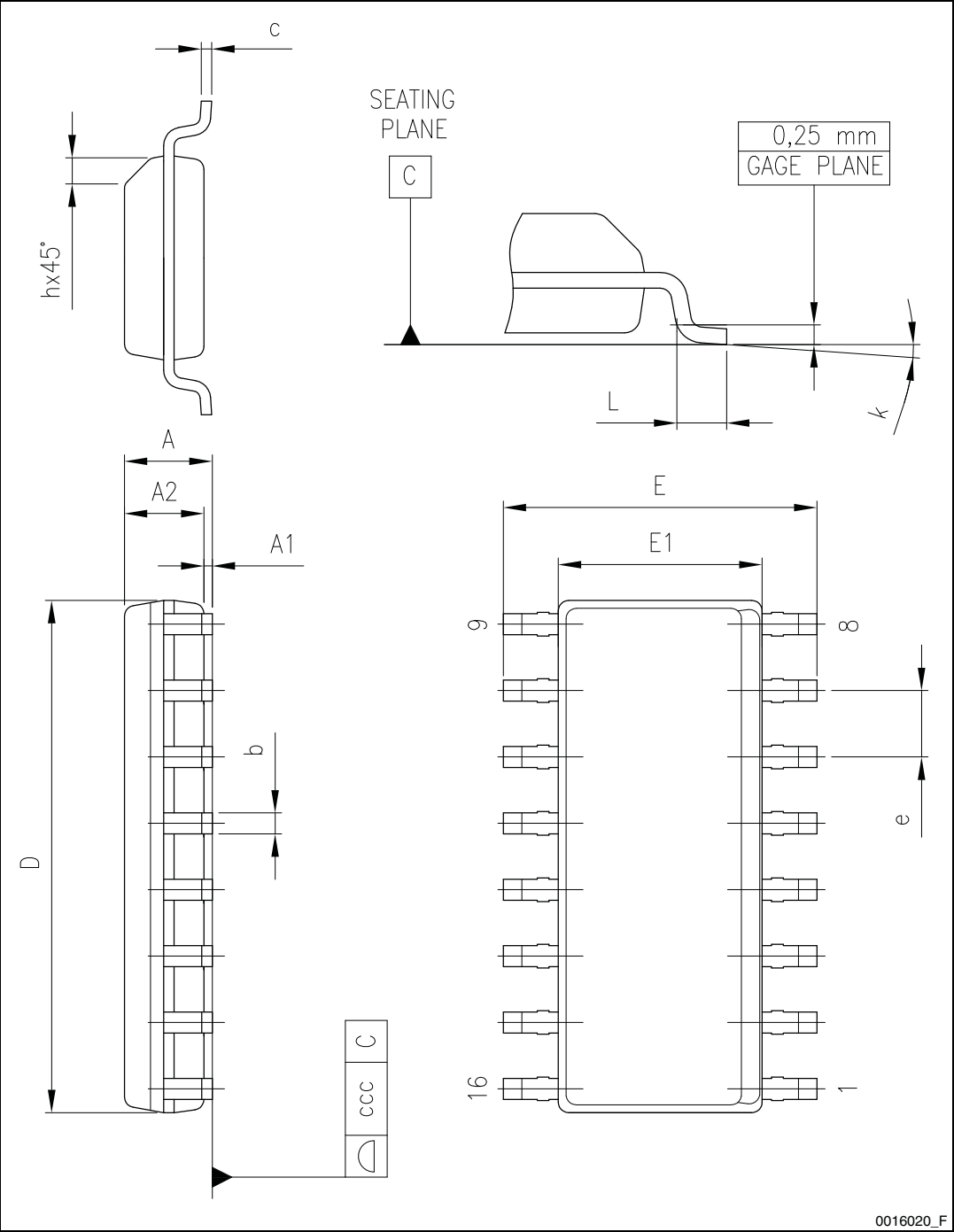
Figure 26. Package drawing
