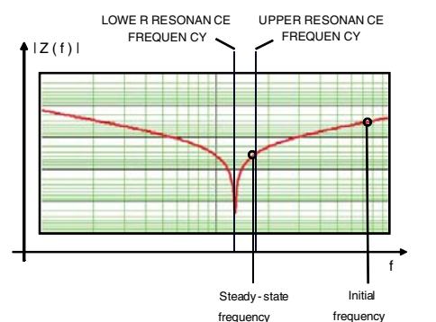
Figure 13. Input impedance vs. frequency curve in an LLC resonant half bridge
