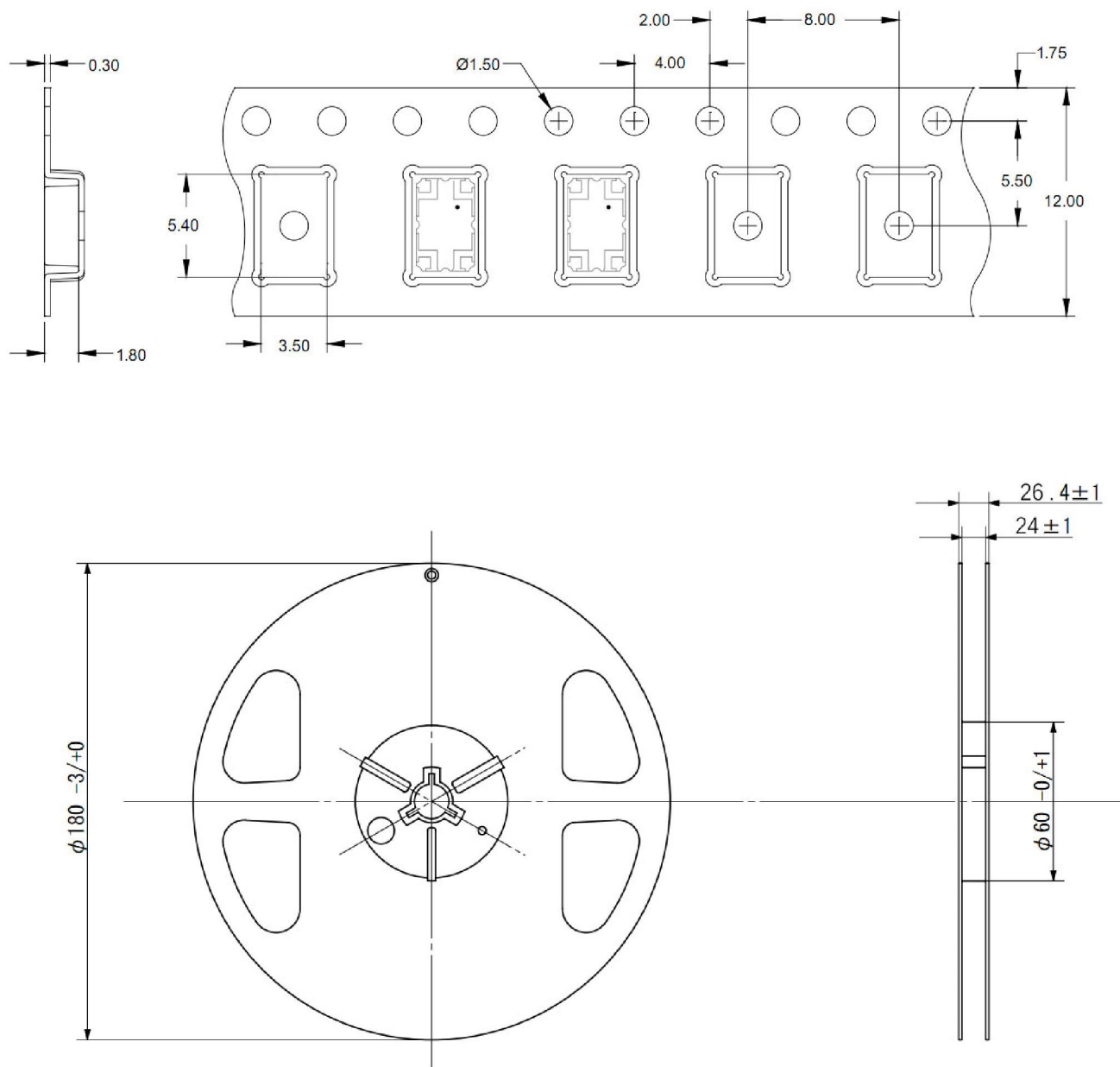
Figure 12. MHC35X03 Packaging Information
