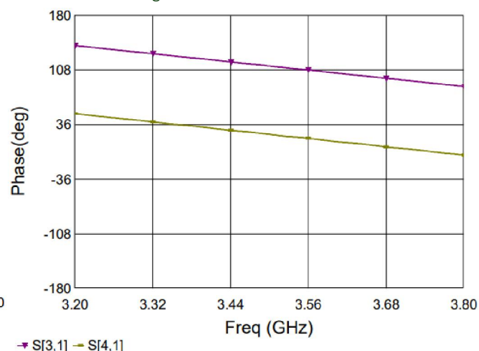
Figure 10. MHC35X03 Phase
