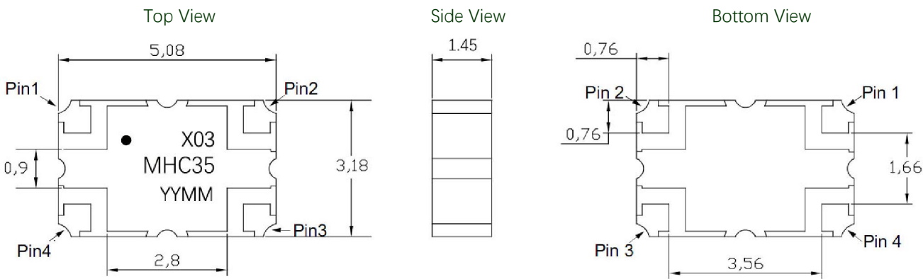
Figure 2. MHC35X03 Outline Drawing
