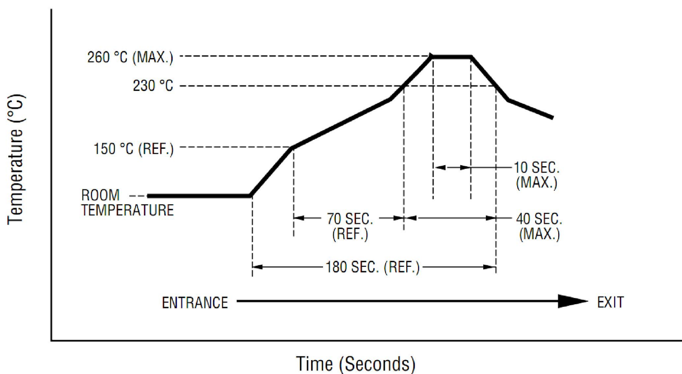
Figure 11. MHC35X03 Thermal Reflow Profile
