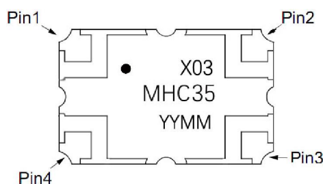
Figure 1. MHC35X03 (Top View)
