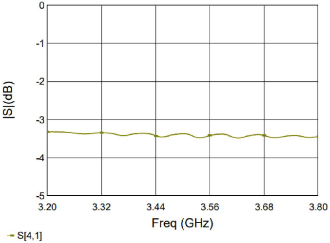
Figure 4. MHC35X03 Transmission
