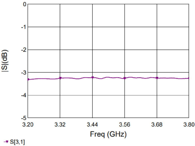
Figure 3. MHC35X03 Coupling
