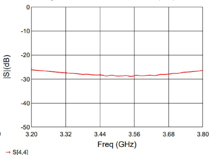
Figure 8. MHC35X03 Return Loss (S44)
