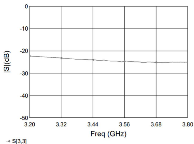
Figure 7. MHC35X03 Return Loss (S33)
