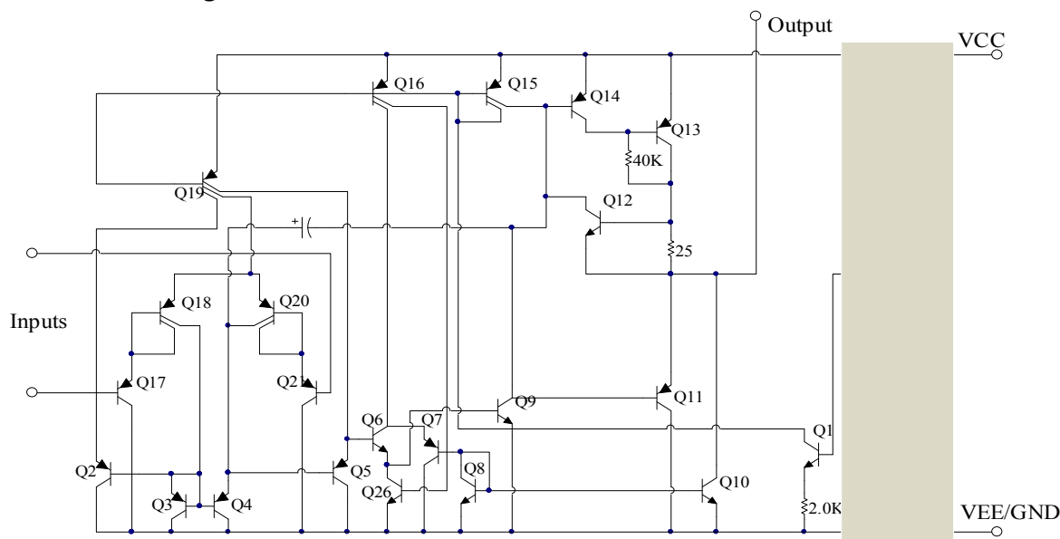
Schematic Diagram (One-Half of Circuit Shown)
