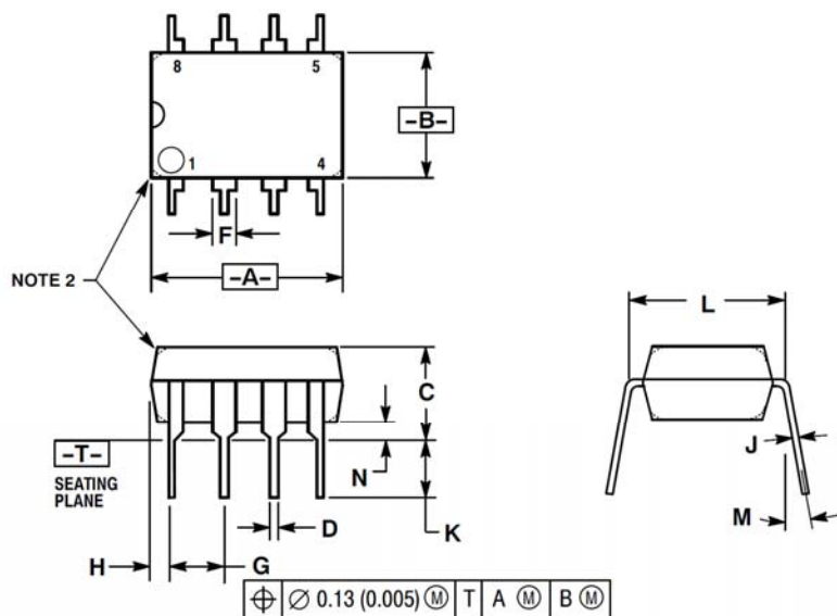
DIP8
