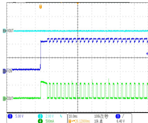
Short-circuit Power-on
